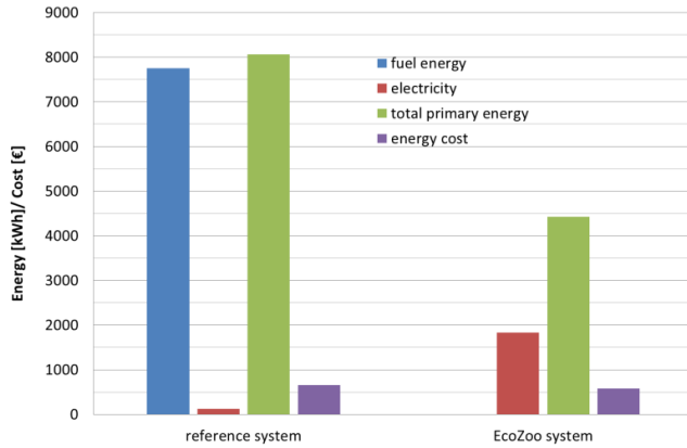
Fig. 7. Comparison between EcoZoo and reference HVAC system: primary energy and energy cost
