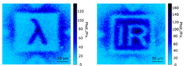
Fig. 3. Silicon “ \lambda ” on a gold background and a gold “IR” on a silicon background. These visible images produced from the infrared illumination correspond to a total accumulation time of 30\ \text{min} .
