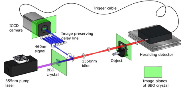
Fig. 1. Experimental setup. The nondegenerate SPDC process generates a visible/infrared photon pair at the BBO crystal, and these photons are split at a dichroic mirror. The infrared photon probes an object and the transmitted photons are detected by a single-element heralding detector (InGaAs/InP single-photon avalanche diode). This detection event triggers the intensifier of the ICCD camera, which detects the delayed yet spatially correlated visible photon. The recovered image of the object is the accumulation of many visible photon detections by the ICCD.
