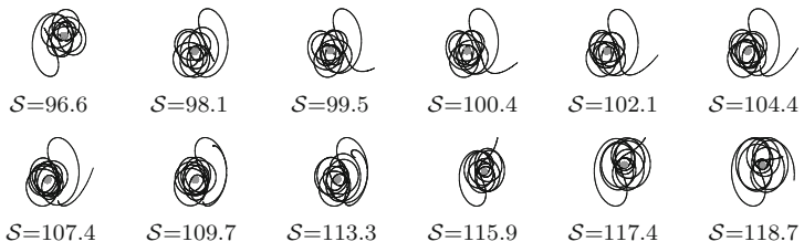
Fig. 12 Ballistic capture orbits about Europa and their stability index in TU
