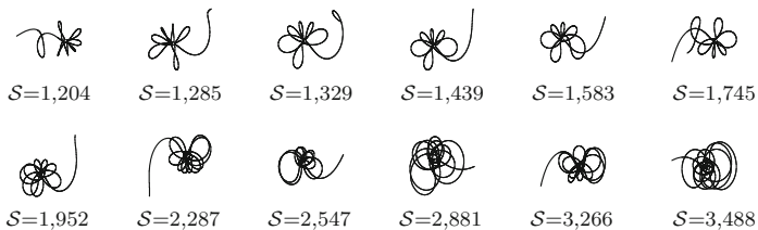
Fig. 8 Ballistic capture orbits about Mercury and their stability index in TU
