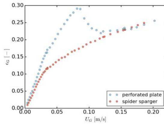
(a) Comparison between coarse and fine gas spargers
