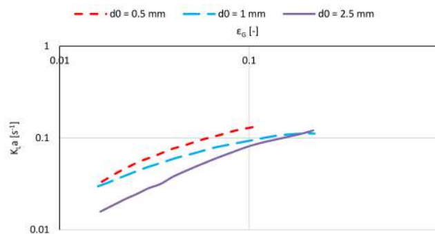
Figure 29. Influence of the gas sparger openings on k_La —data taken from Koide et al. [138].
