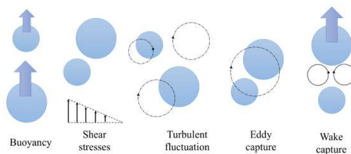
Figure 40. Coalescence mechanisms.
