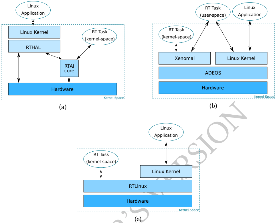
Fig. 1. The three different implementations of the co-kernel approach: (a) RTAI, (b) Xenomai, (c) RTLinux
