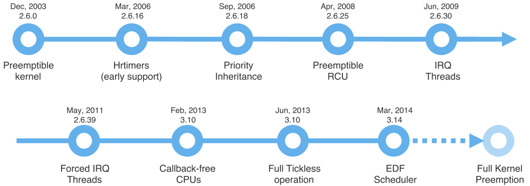
Fig. 2. Timeline of merged real-time features in the mainline Linux kernel, most of them coming from PREEMPT_RT patch.
