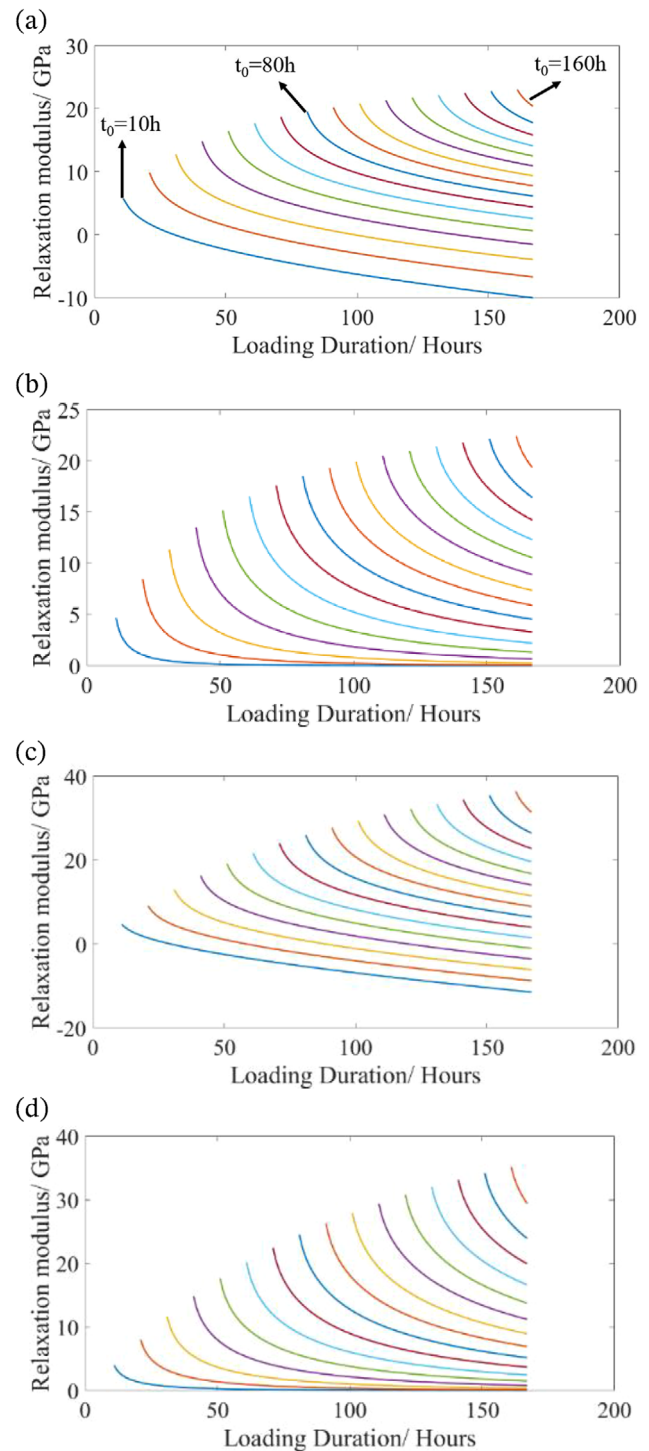
FIGURE 13 Relaxation modulus R(t_0, t) : (a) C1 results by M1, (b) C1 results by M2, (c) C3 results by M1, and (d) C3 results by M2. (Note that the results displayed here are R(t_0, t) with t_0 equal to 10, 20, 30, ..., and 160 h. See (a) for the example.)
