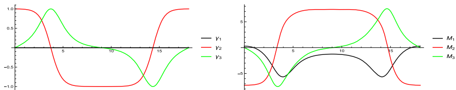
Fig. 6 Components \gamma_j (left) and M_j (right) for the first orbit described in Theorem 3.1
