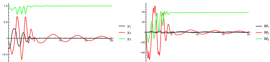
Fig. 3 Components \gamma_j (left) and M_j (right) for the first orbit described in Theorem 2.2
