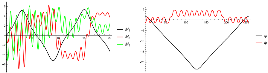
Fig. 5 Components M_j (left) and angles \psi, \phi (right) for the orbit described in Theorem 2.3
