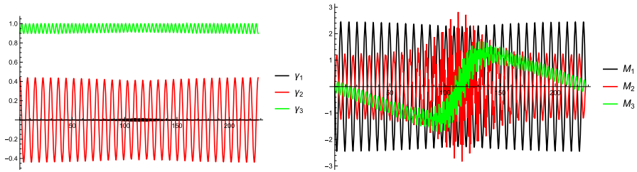
Fig. 2 Components \gamma_j (left) and M_j (right) for the orbit described in Theorem 2.1
