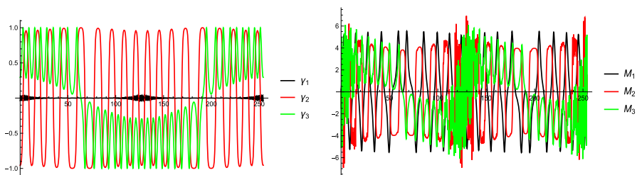
Fig. 4 Components \gamma_j (left) and M_j (right) for the orbit described in Theorem 2.3
