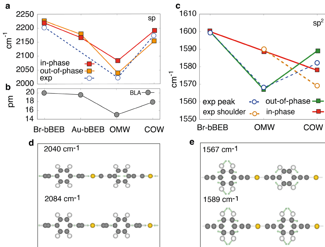
Fig. 7 Frequencies, calculated and measured (a) and bond length alternation (b) of -C\equiv C- stretching modes in freestanding OMWs. Red: in phase -C\equiv C- stretching mode, orange: out of phase -C\equiv C- stretching mode, blue: experimental fit of the Raman peak frequencies. (c) Calculated and measured frequencies of modes involving benzene rings. Red: in phase-benzene breathing mode, green: out of phase benzene breathing mode, blue: experimental fit of the main Raman peak, orange: experimental fit of the Raman shoulders nearby the main peak representing the softening of the "in phase" vibrational mode during the OMW-to-COW transition. (d and e) Atomic displacements of the symmetric "in phase" and antisymmetric "out of phase" phonon modes of OMWs (phonon modes of other species are reported in SI). Experimental data are extracted from Fig. 6.
