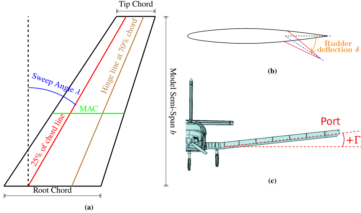
Fig. 1 Planform definition of a trapezoidal lifting surface: (a) in-plane parameters, (b) rudder deflection definition, (c) dihedral angle.
