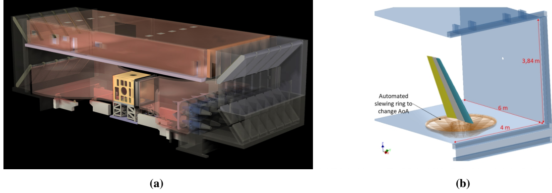
Fig. 5 The large wind tunnel of Politecnico di Milano (GVPM): (a) general layout of GVPM; (b) tail-plane model installed in the wind tunnel.
