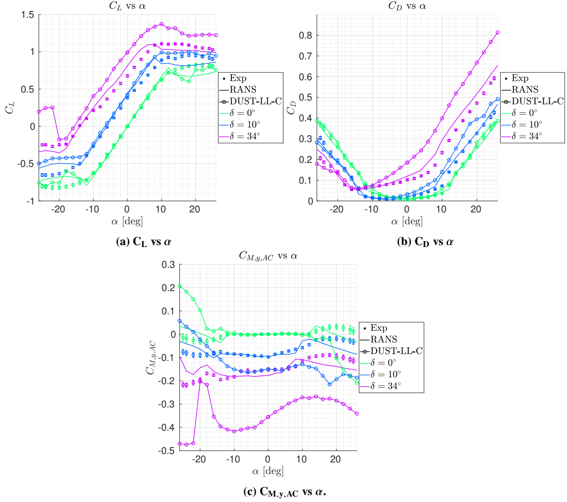
Fig. 8 Comparison between Wind Tunnel, RANS, and Lifting Line method results in terms of the aerodynamic coefficients for \Gamma = 0 deg.
