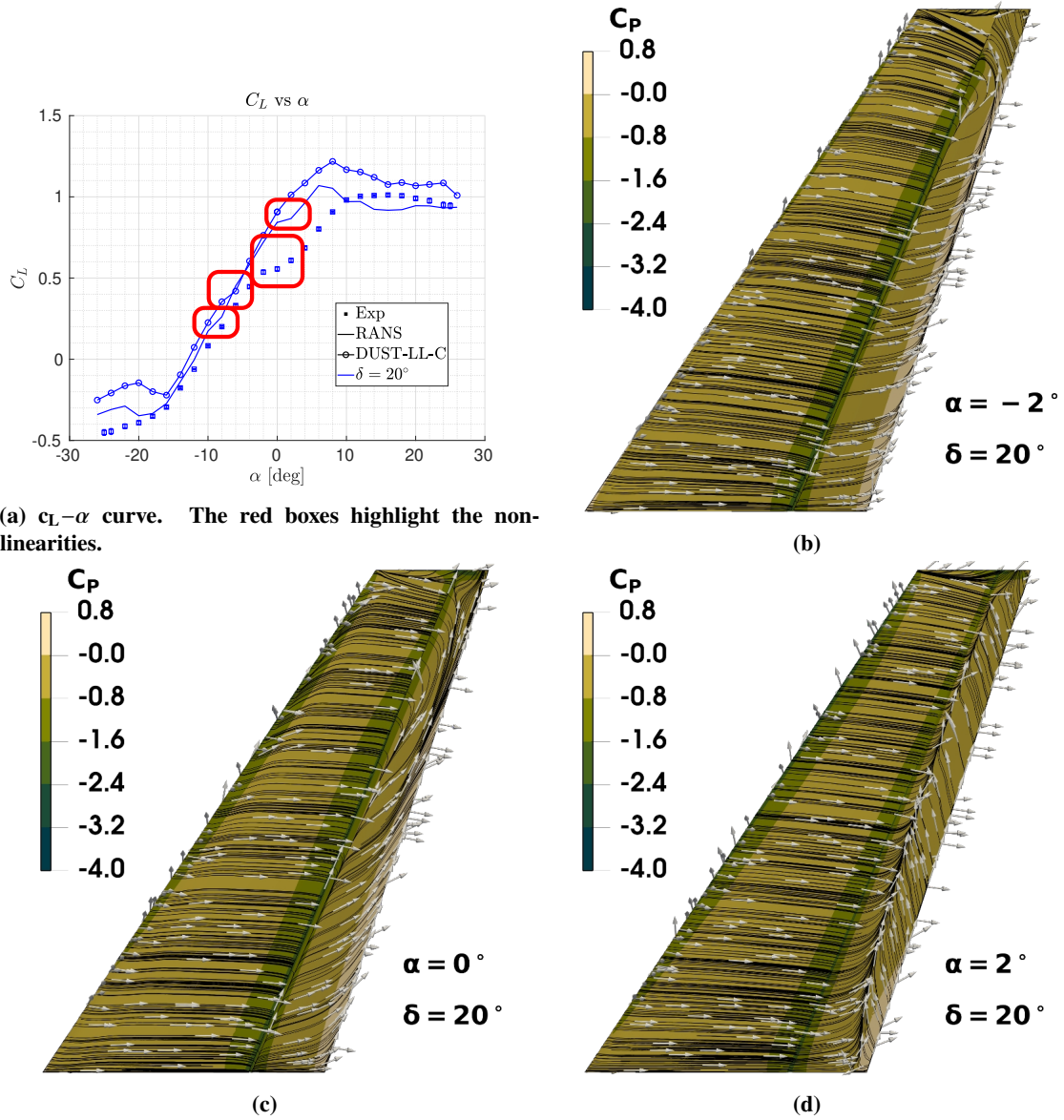
Fig. 11 Stall visualization at the control surface for \Gamma=0 deg, \delta=20 deg: (a) lift curve, (b–d) pressure distribution and skin-friction streamlines.
