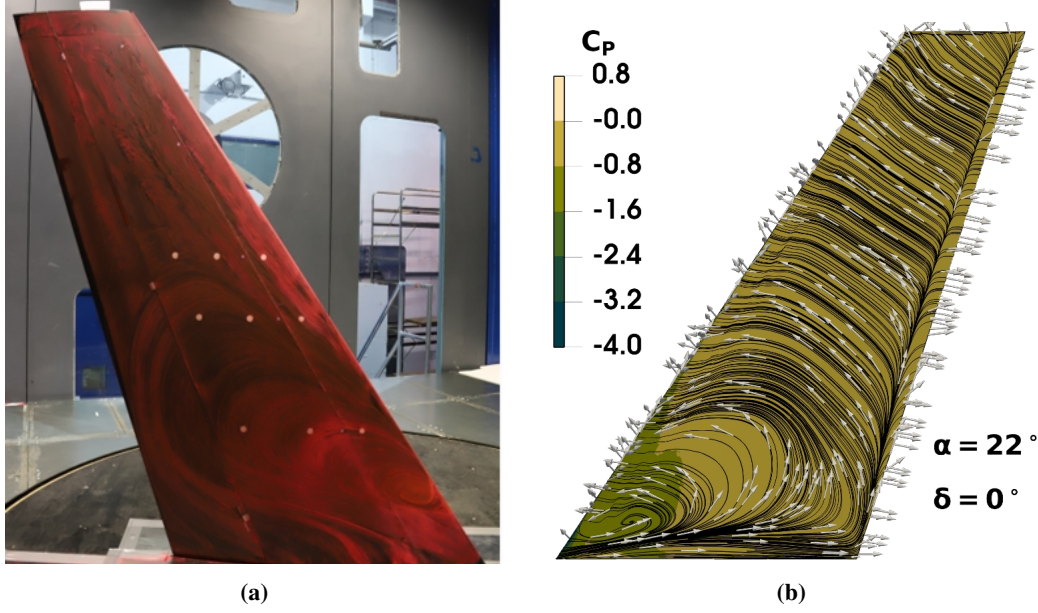
Fig. 10 Comparison of the spanwise location of the vortex locus on the suction side of the model: (a) experimental china-clay flow visualization, and (b) numerical RANS results with surface streamlines aligned with the skin-friction coefficient and colored by the pressure coefficient.
