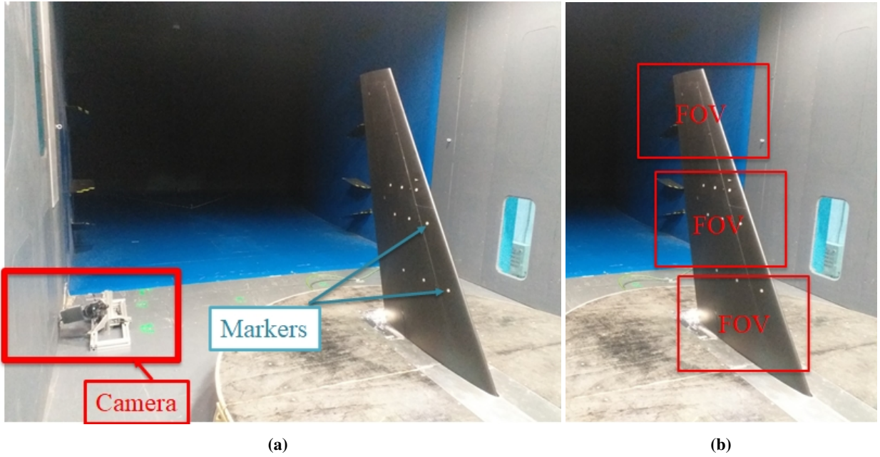
Fig. 6 Set-up of the infrared thermography instrumentation: (a) camera position and reference markers, (b) field of views (FOV) of the infrared thermography measurements.
