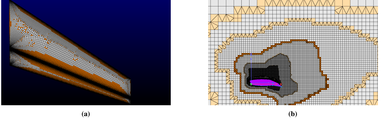
Fig. 3 Visualization of employed meshing strategies: (a) surface mesh, (b) volume mesh.
