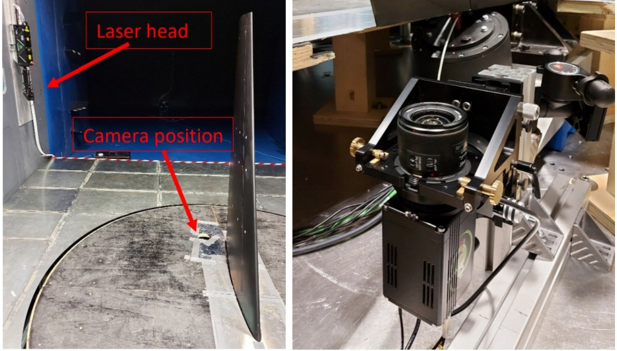
Fig. 7 PIV surveys: laser and camera installation.
