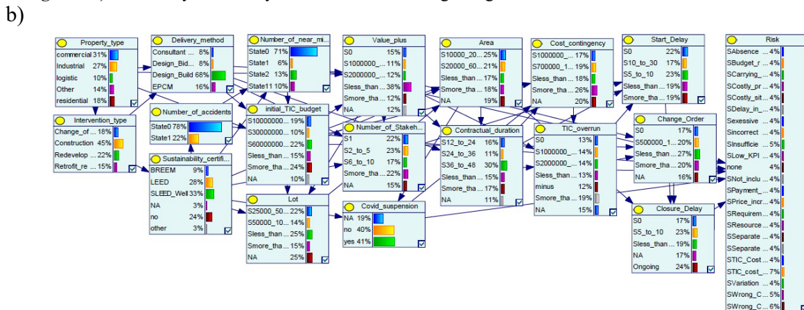
Figure 6b) Case study Bayesian Search Network for all financial risks' identification
