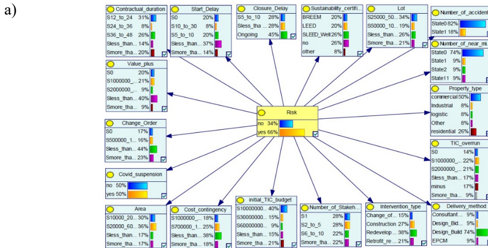
Figure 6a) Case study Naïve Bayes Network for “Wrong Budget Estimation” financial risk identification
