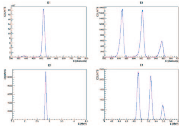
Fig. 2. – Comparison between experimental (higher panels) and simulated data (lower panels) for the 10\text{ }\mu\text{m} (left) and 100\text{ }\mu\text{m} (right) thick detector for just one of the four pads, with the two different \alpha -sources ( ^{148}\text{Gd} left, 3-peaks \alpha -source right).
