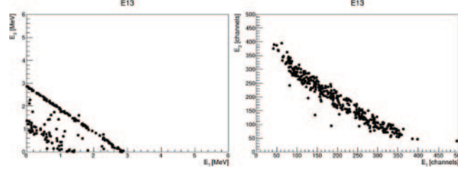
Fig. 3. – Interpad events comparison between simulations (left panel) and experimental data (right panels) for the 10 \mu\text{m} thick detector for two adjacent pads (coincidences events, ^{148}\text{Gd} \alpha -source).
