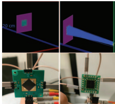
Fig. 1. – Upper panels: SiC geometry as simulated by means of Geant4; lower panels: pictures of SiC with same surface and different thicknesses (100 \mu\text{m} left, 10 \mu\text{m} right).
