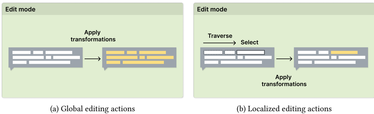
Figure 4: Editing actions
