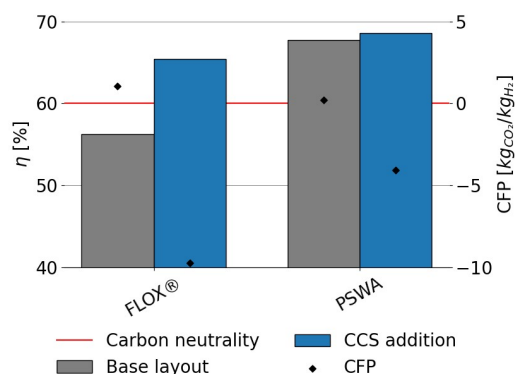
Fig. 9 Energy efficiency and fossil carbon footprint of biogas conversion to hydrogen using Italian grid as source of electricity.
