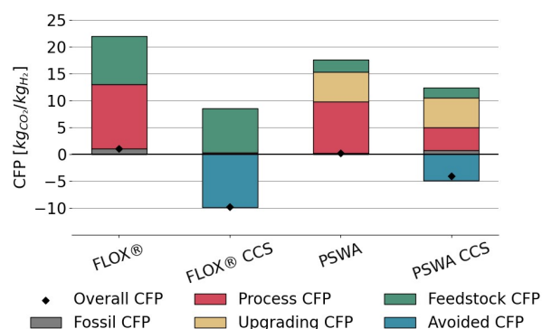
Fig. 10 Carbon footprint derived from biogas conversion to hydrogen using Italian grid as source of electricity. The feedstock CFP is the CO 2 from biogas that is emitted. The process CFP is the CO 2 formed in the process (e.g., by combustion), but of biogenic source. The upgrading CFP is the CO 2 removed by scrubbing for biogas upgrading and released in the atmosphere according to this analysis.
