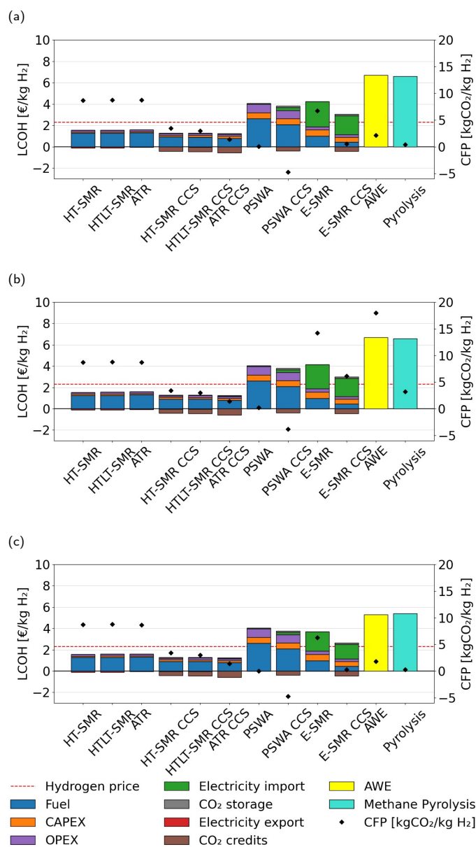
Fig. 14 Scenario-based LCOH assessment with the use of (a) Swiss grid, (b) German grid and (c) French grid for the electric supply to the processes. The red dotted line defines the threshold hydrogen market value averaged from the reference database 87 .
