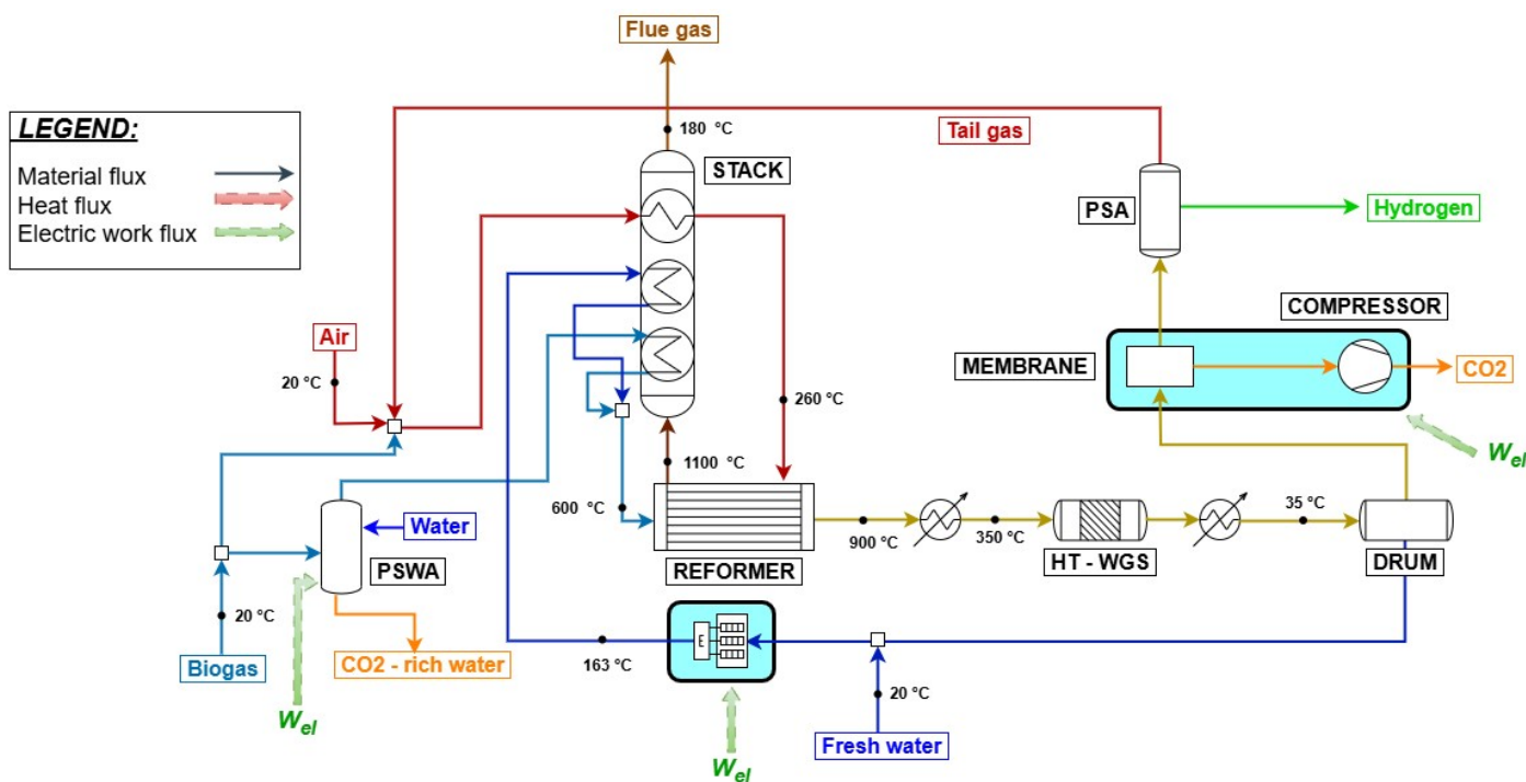
Fig. 5 Biogas steam reforming with PSWA biogas scrubbing and CCS unit.
