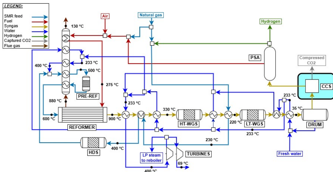
Fig. 2 Natural gas steam reforming plant scheme with HT + LT-WGS and CCS unit, whose addition is highlighted.
