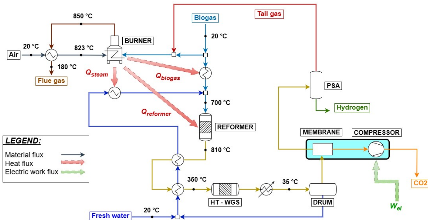
Fig. 4 Biogas steam reforming through FLOX ® with CCS unit and PSA hydrogen separation.
