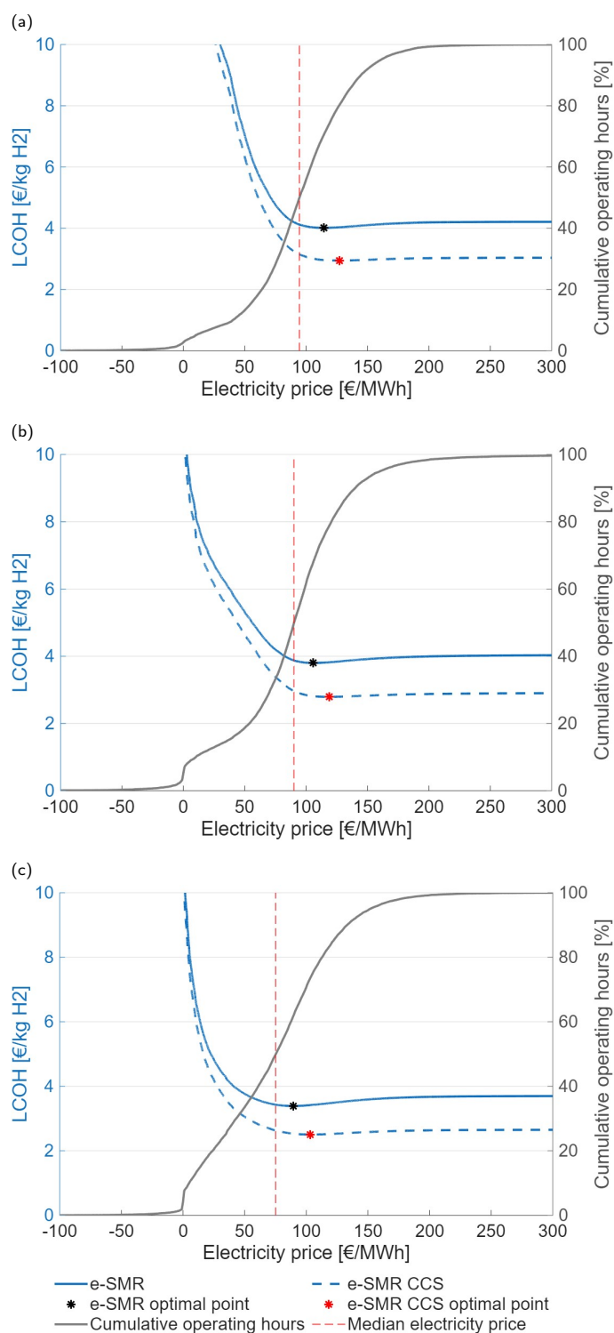
Fig. 16 Scenario-based dynamic LCOH assessment with the use of (a) Swiss grid, (b) German grid and (c) French grid for the electric supply to the processes.
