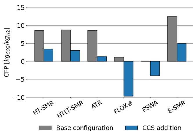
Fig. 13 Overall comparison of the carbon footprint of the processes assessed through this work. Electricity supply is assumed to be achieved through Italian national grid.
