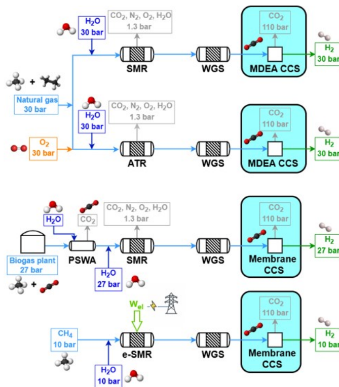
Fig. 1 Visualization of the plant battery limits. The CCS unit is highlighted, as it is optional in the plant layout.
