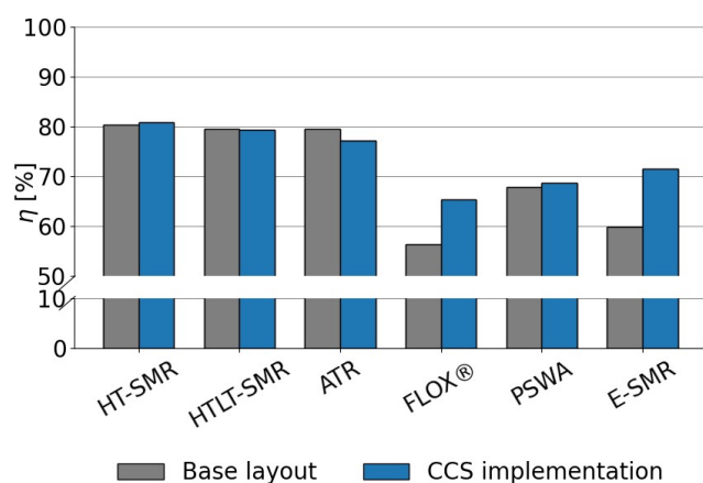
Fig. 12 Overall comparison of the energy efficiency of the processes assessed through this work.
