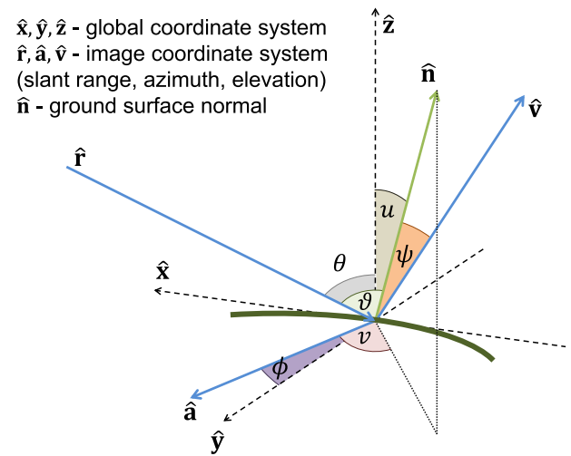
Fig. 1. Geometry of the data acquisition for a left-looking SAR system: \phi is the flight heading angle, \theta is the global incidence angle, \vartheta is the local incidence angle, and u and v are the ground slope and slope aspect angles. The angle between the image surface normal and the ground surface normal is referred to as \psi and is used for accurate calibration to \sigma^0 (Ulander, 1996).
