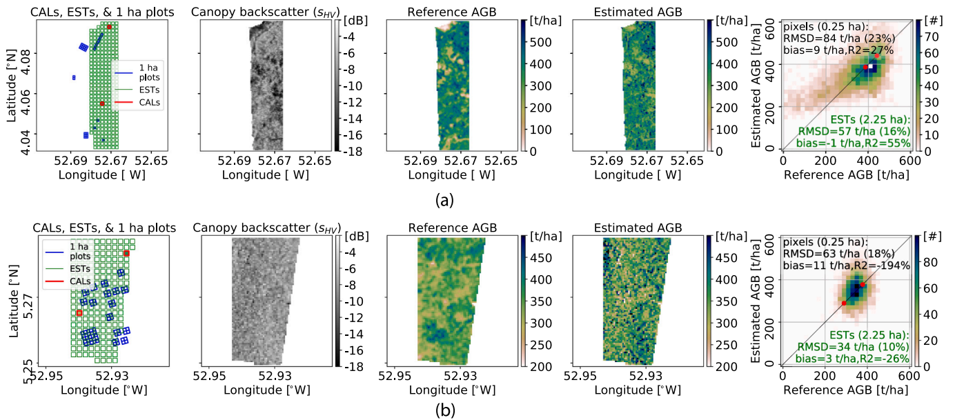
Fig. 6. Best-case AGB estimation results in (a) Nouragues and (b) Paracou, in French Guiana. The leftmost plots show the 150 m × 150 m estimation (EST) areas, two 150 m × 150 m calibration (CAL) areas, and the 1 ha in situ plots. The next three plots show the canopy backscatter for HV polarisation ( S_{HV} ), the reference AGB map from ALS data, and the best-case AGB map estimated from SAR with CASINO. The rightmost plots show 2D histograms created using all pixels from the reference and estimated AGB maps, with the colour scale indicating the number of pixels; these plots include performance metrics for the 2.25 ha EST areas (bottom right corner) and the 0.25 ha pixels (top left corner). The red dots in the scatterplots show estimation results for the two CAL areas. The SAR data were acquired with the left-looking SETHI system.
