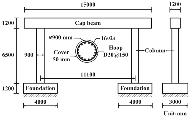
Fig. 12. Detailed dimensions of the bridge pier.
