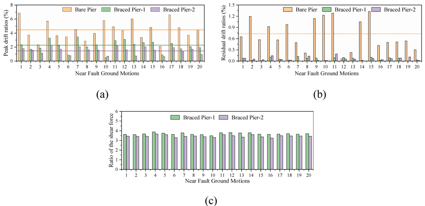
Fig. 20. Comparison of three types bridge piers response under 20 ground motions: (a) peak drift ratios, (b) residual drift ratios and (c) peak base shear force.
