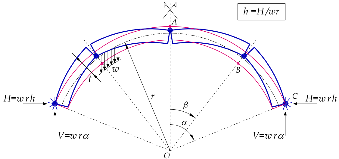
Fig. 2. Least-thickness “Couplet–Heyman problem”. Purely-rotational collapse mode, with shoulder-hinge reactions V and H (opposite of weight of half-arch and horizontal thrust). Characteristic variables: angular inner-hinge position \beta = \beta_r , thickness-to-radius ratio \eta = t/r and non-dimensional horizontal thrust h = H/(wr) .
