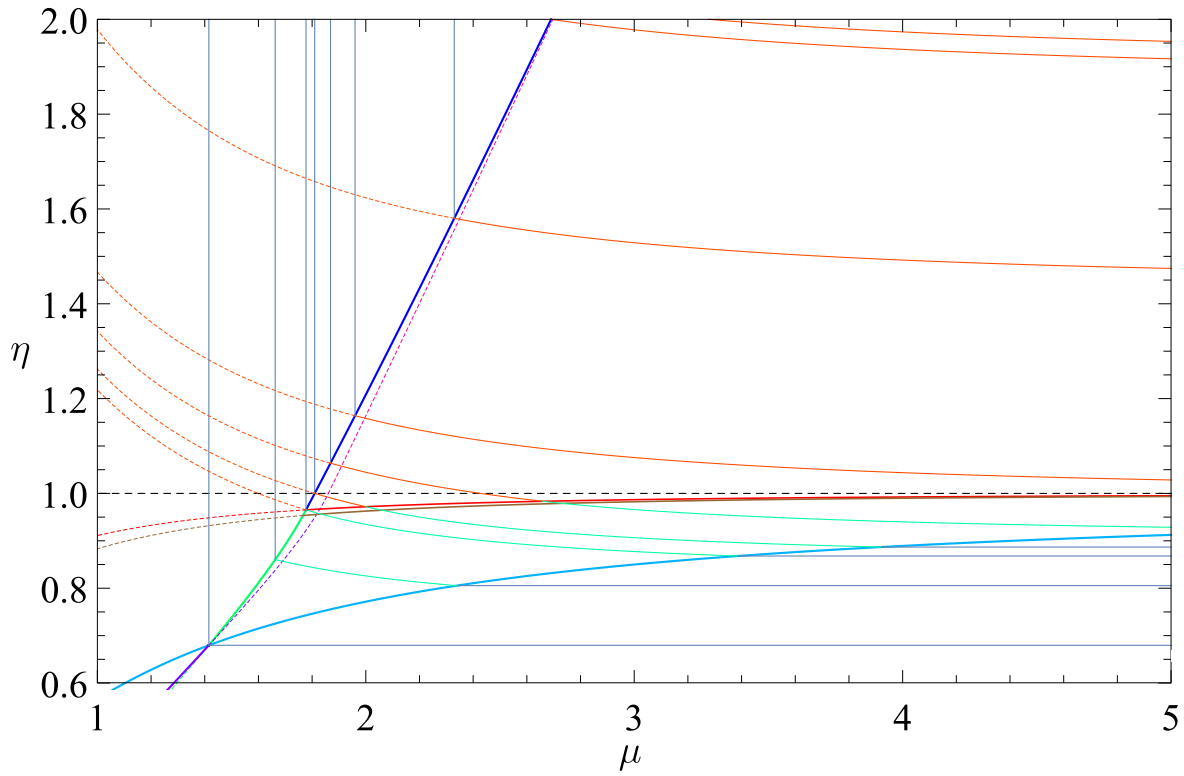
Fig. 8. Analytical \eta - \mu map of self-standing and collapse states: 0.6 \leq \eta \leq 2 zoom.
