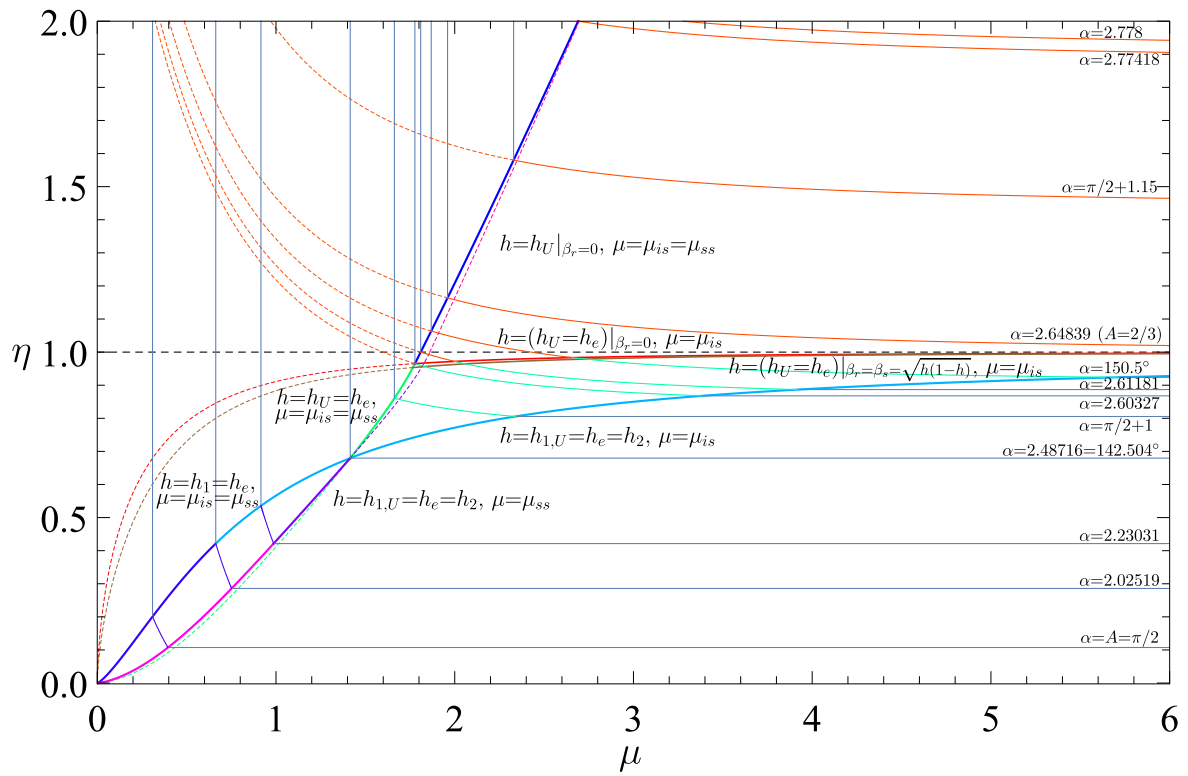
Fig. 6. Analytical \eta - \mu map of self-standing and collapse states, for all admissible 0 \leq \eta \leq 2 .
