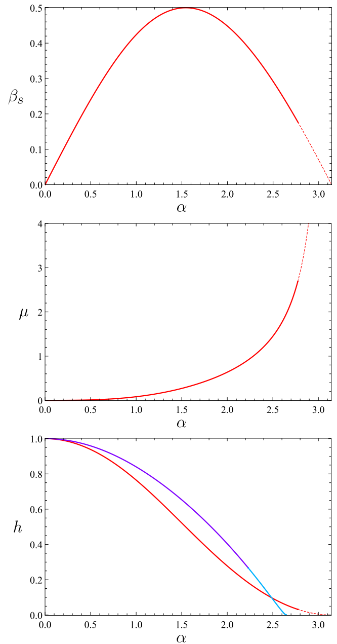
Fig. 5. Purely-sliding solution for triplet \beta = \beta_s , \mu , h as a function of \alpha .
