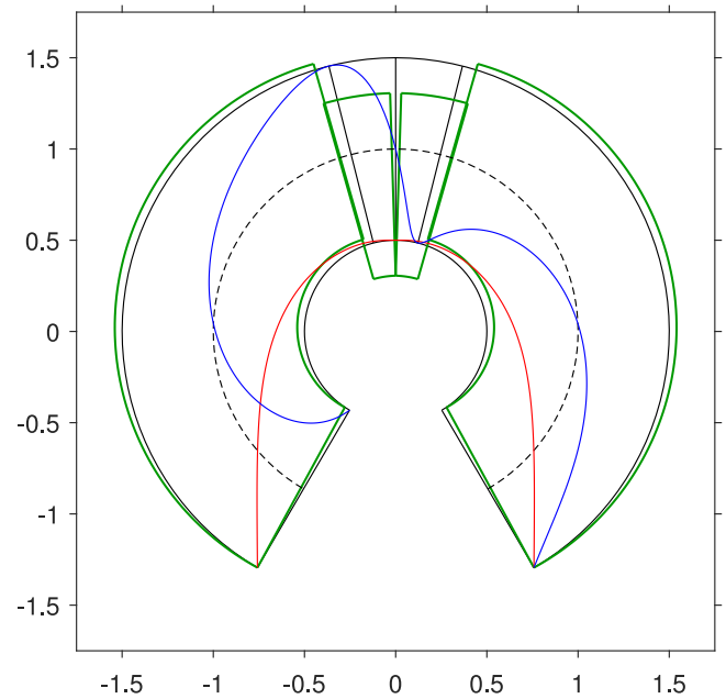
Fig. 23. Least-thickness collapse mechanism, with line of thrust and line of friction: at point with \alpha = 2.611810358168302 \approx 149.6^\circ , \mu = 1.809583028035458 ( \varphi \approx 61.1^\circ ), \eta = 1 : purely-sliding (top); overturning-sliding (low).
