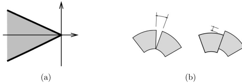
Fig. 12. (a) Strength conditions within static internal variables \varphi \leq 0 ; (b) Collapse kinematic variables at rotating/sliding joints \dot{\lambda} \geq 0 .
