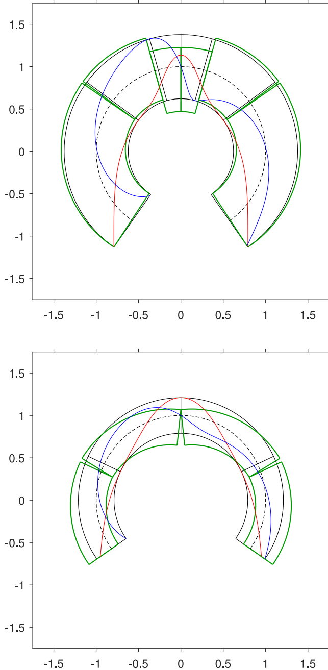
Fig. 17. Least-thickness collapse mechanism, with line of thrust and line of friction: (top) rotational-sliding, for \alpha = 145^\circ , \mu = 1.6 ( \varphi \simeq 58.0^\circ ), \eta = 0.7566761737936022 ; (low) sliding-rotational, for \alpha = 125^\circ , \mu = 0.9 ( \varphi \simeq 42.0^\circ ), \eta = 0.4208869235292454 .
