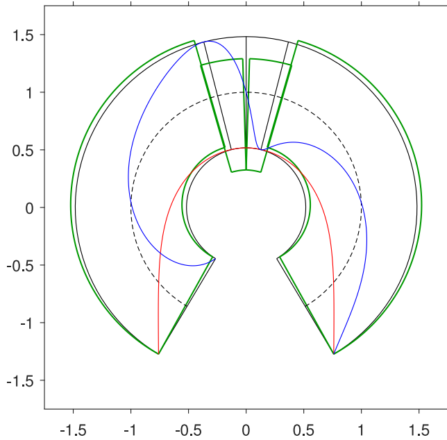
Fig. 20. Least-thickness collapse mechanism, with line of thrust and line of friction: at “Junction point” with \alpha_J = 2.603266515104794 \simeq 149.2^\circ , \mu_J = 1.777213608388235 ( \varphi_J \simeq 60.6^\circ ), \eta_J = 0.9652414772084198 : purely-sliding (top); rotational(overturning)-sliding (low).
