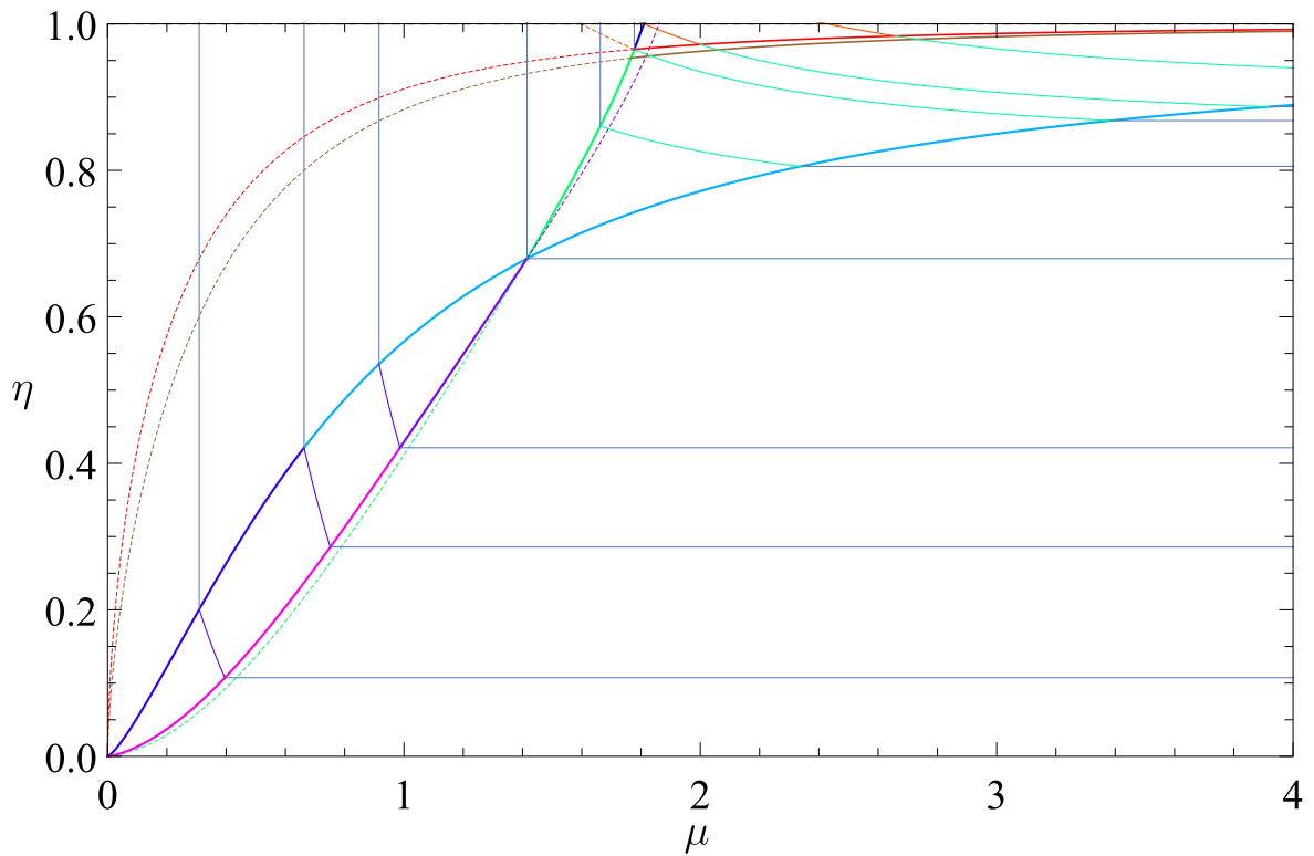
Fig. 7. Analytical \eta - \mu map of self-standing and collapse states: 0 \leq \eta \leq 1 zoom.
