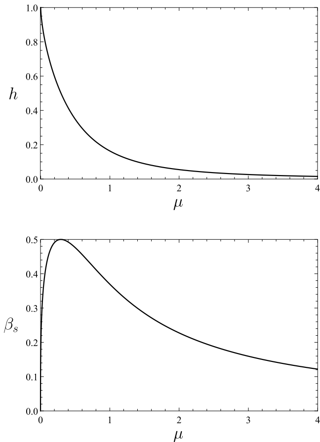
Fig. 4. Relations h of \mu (top) and \beta_s of \mu (low) at inner sliding activation.
