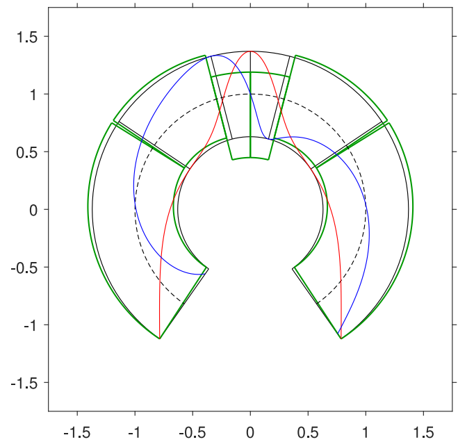
Fig. 16. Least-thickness collapse mechanism, with line of thrust and line of friction: (top) rotational-sliding, for \alpha = 145^\circ , \mu = 1.536310506737699 ( \varphi \simeq 56.9^\circ ), \eta = 0.7643357111953571 ; (low) rotational-sliding, for \alpha = 145^\circ , \mu = 1.761938080825641 ( \varphi \simeq 60.4^\circ ), \eta = 0.7406376307743147 .
