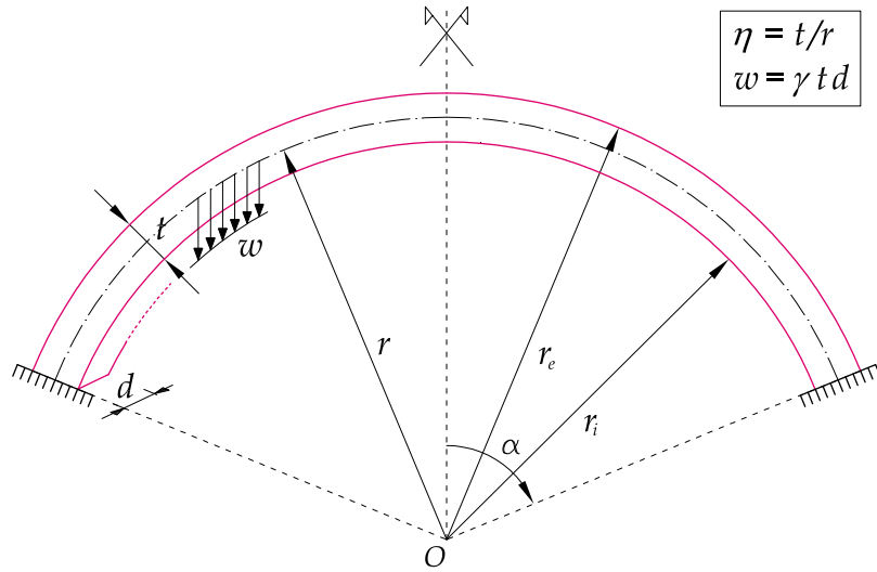
Fig. 1. Symmetric circular masonry arch under self-weight ( \gamma specific weight per unit volume) with involved characteristic parameters ( d out-of-plane depth).
