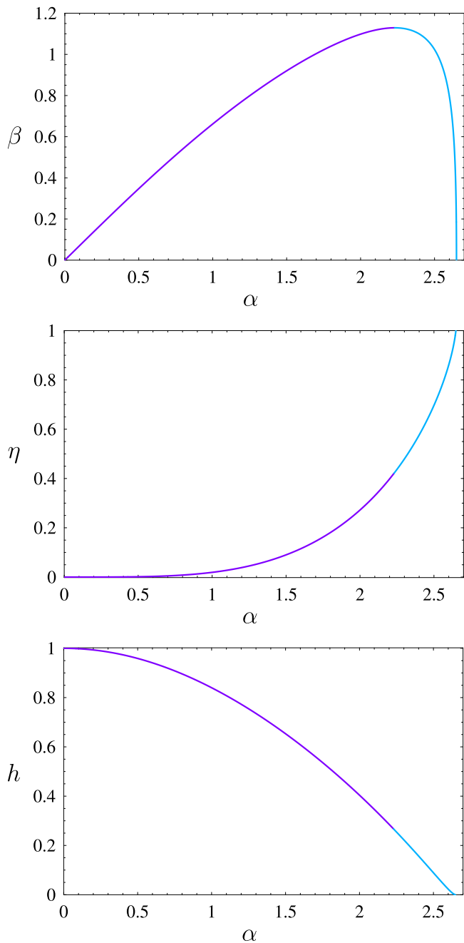
Fig. 3. Purely-rotational least-thickness solution for triplet \beta = \beta_r, \eta, h as a function of \alpha .
