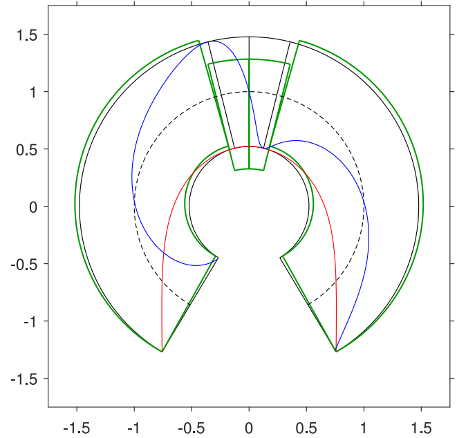
Fig. 21. Least-thickness collapse mechanism, with line of thrust and line of friction: at \alpha_J = 2.603266515104794 \simeq 149.2^\circ (rotational-sliding): \mu = 1.79 ( \varphi \simeq 60.8^\circ ), \eta = 0.9630759684607590 ( \beta_r < \beta_s , top); \mu = 1.832508693777595 ( \varphi \simeq 61.4^\circ ), \eta = 0.9563124518512550 ( \beta_r = \beta_s , low).
