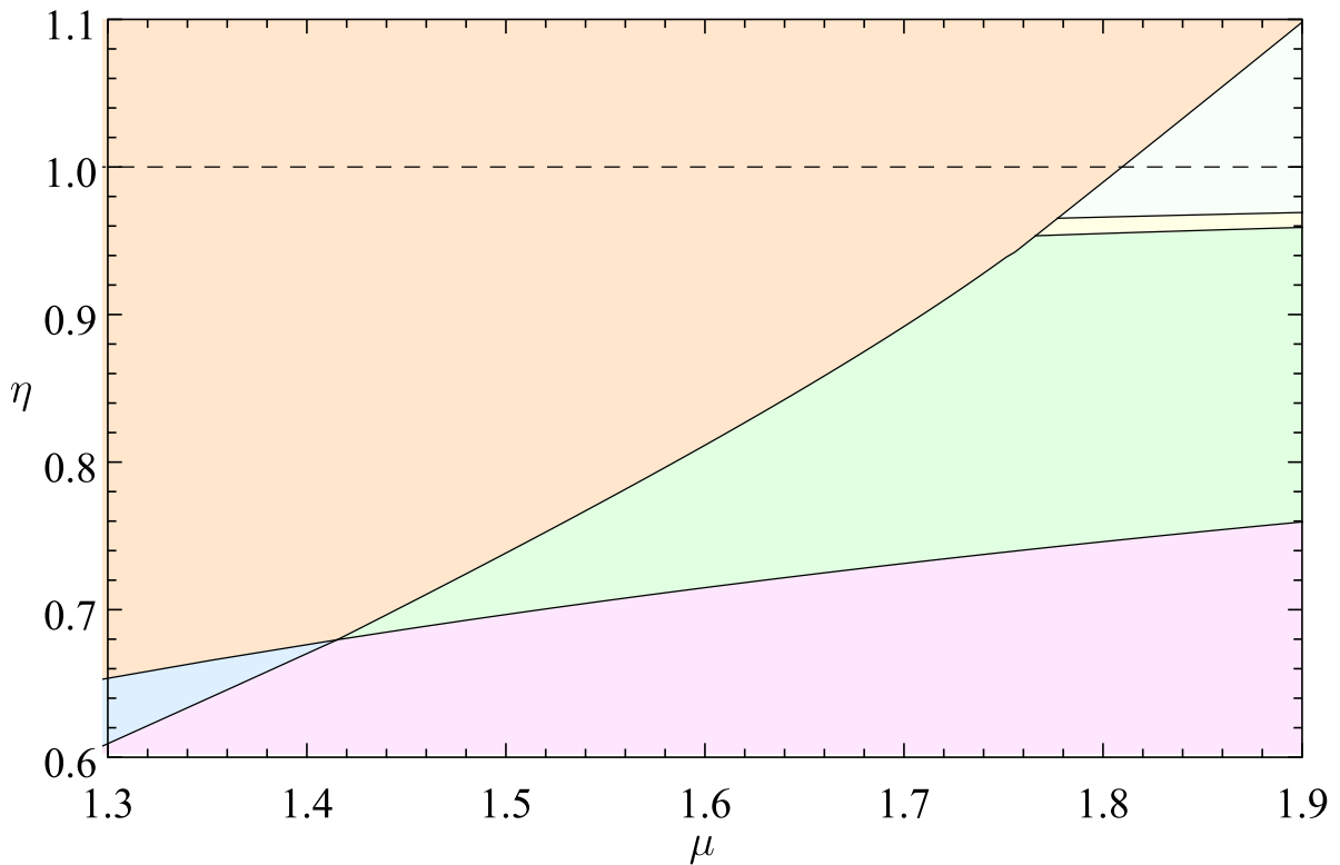
Fig. 11. Filled \eta - \mu domains of self-standing and collapse states: central zoom.
