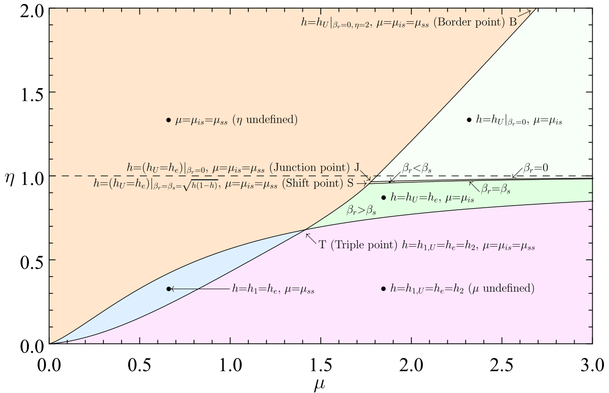
Fig. 9. Analytical \eta - \mu domains of self-standing and collapse states.
