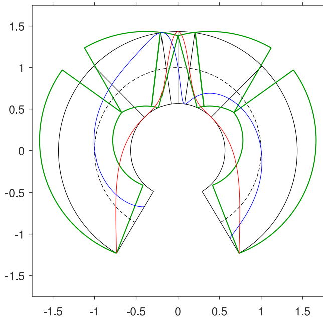
Fig. 22. Least-thickness collapse mechanism, with line of thrust and line of friction: at point with \alpha_f = 2.603266515104794 \approx 149.2^\circ , \mu = 3.385846504480999 ( \varphi \approx 73.6^\circ ), \eta = 0.8679273523649103 : rotational-sliding ( \beta_r > \beta_s , top); purely-rotational (low).
