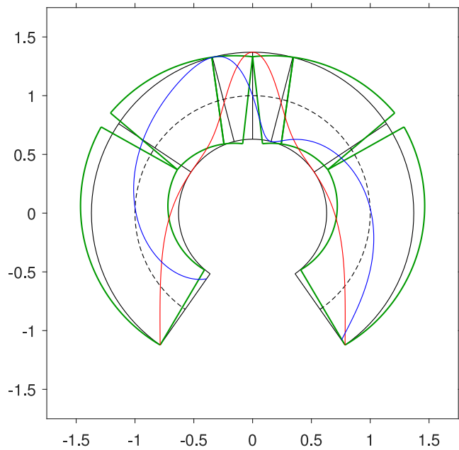
Fig. 15. Least-thickness collapse mechanism, with line of thrust and line of friction: (top) purely-sliding, for \alpha = 145^\circ , \mu = 1.536310506737699 ( \varphi \simeq 56.9^\circ ), \eta = 0.7643357111953571 ; (low) purely-rotational, for \alpha = 145^\circ , \mu = 1.761938080825641 ( \varphi \simeq 60.4^\circ ), \eta = 0.7406376307743147 .
