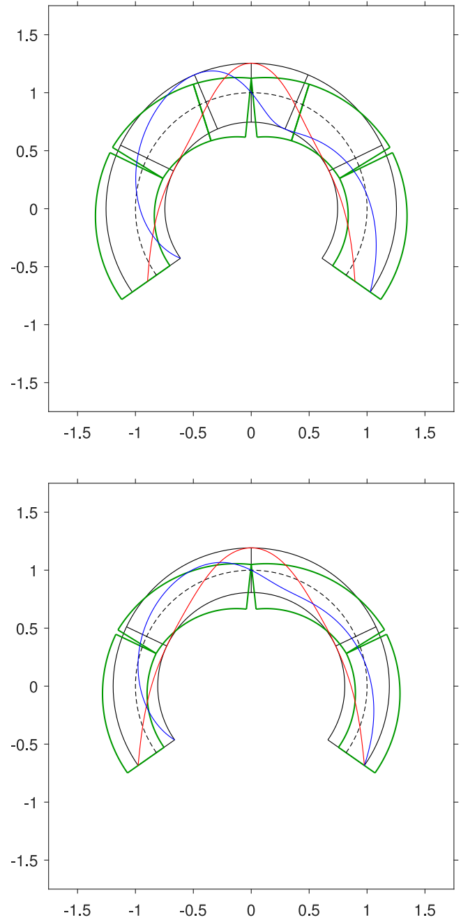
Fig. 14. Least-thickness collapse mechanism, with line of thrust and line of friction: (top) sliding-rotational, for \alpha = 125^\circ , \mu = 0.8477497839674316 ( \varphi \simeq 40.3^\circ ), \eta = 0.5081418006878796 ; (low) sliding-rotational, for \alpha = 125^\circ , \mu = 0.9245590639478306 ( \varphi \simeq 42.8^\circ ), \eta = 0.3849612500740051 .
