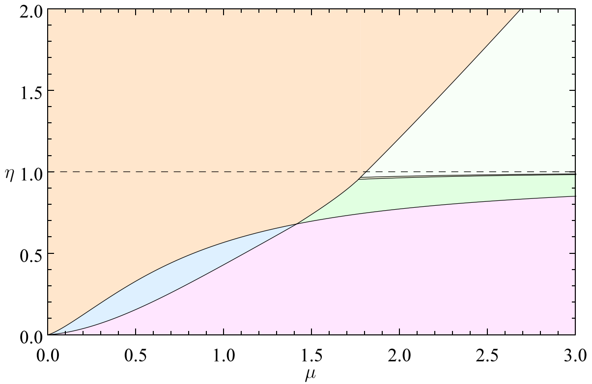
Fig. 10. Filled \eta - \mu domains of self-standing and collapse states.
