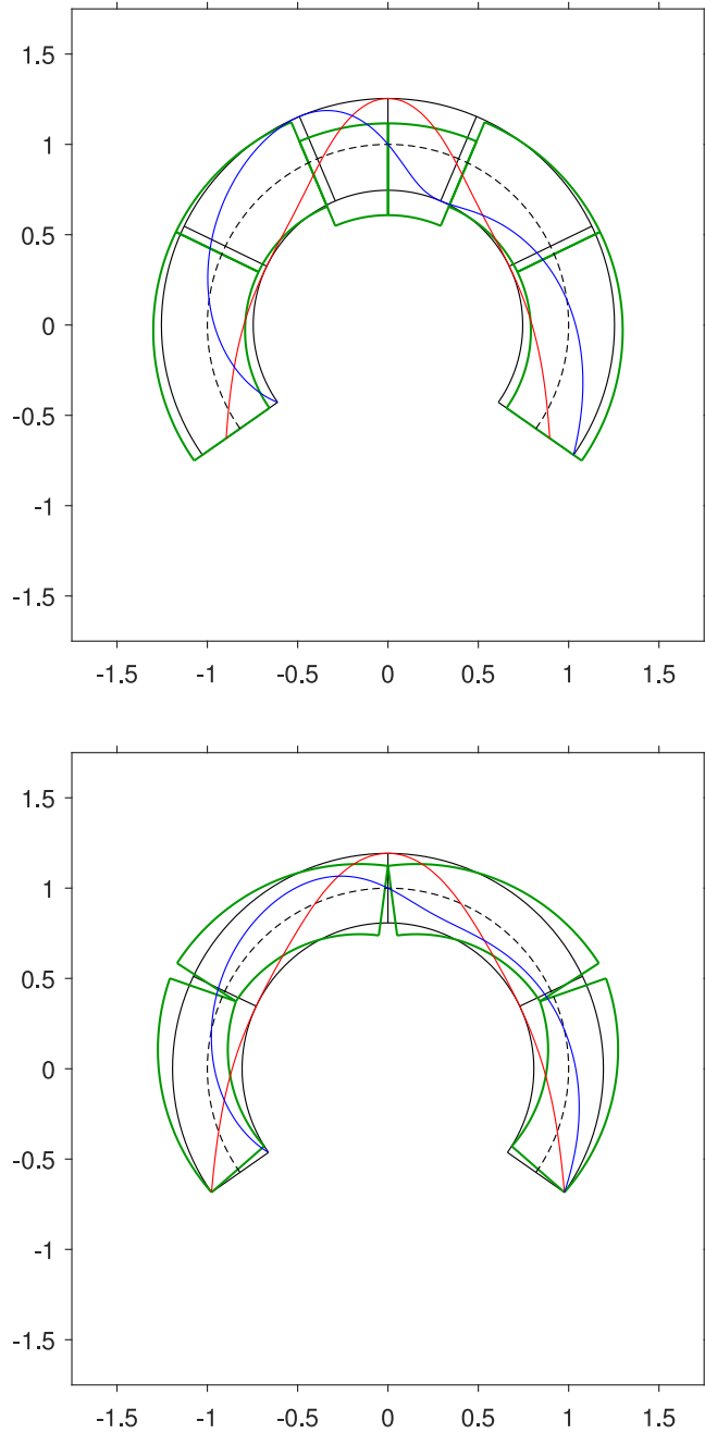
Fig. 13. Least-thickness collapse mechanism, with line of thrust and line of friction: (top) purely-sliding, for \alpha = 125^\circ , \mu = 0.8477497839674316 ( \varphi \simeq 40.3^\circ ), \eta = 0.5081418006878796 ; (low) purely-rotational, for \alpha = 125^\circ , \mu = 0.9245590639478306 ( \varphi \simeq 42.8^\circ ), \eta = 0.3849612500740051 .
