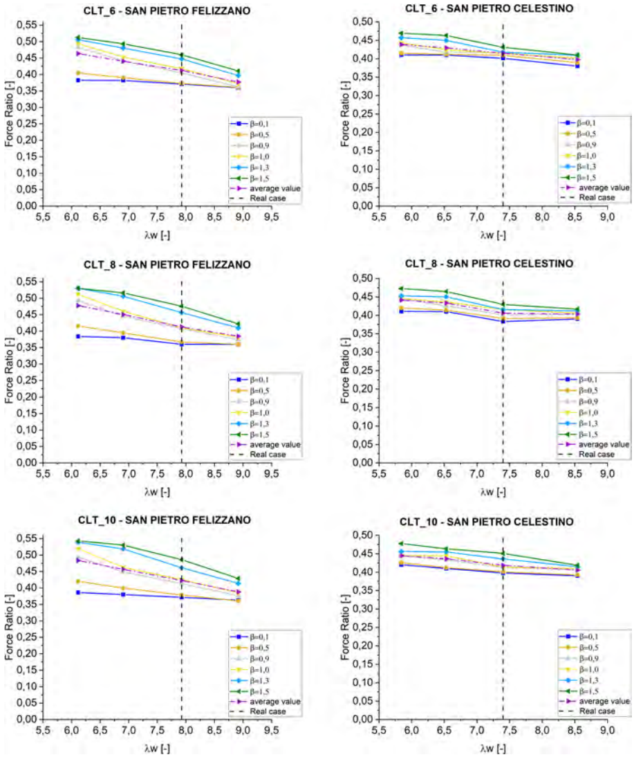
Fig. 15 force ratio (base shear/axial force on the facade) for San Pietro Felizzano and San Pietro San Pietro Celestino in relation to the geometrical slenderness of the lateral walls ( \lambda w ) for the three different CLT roof structure configurations
