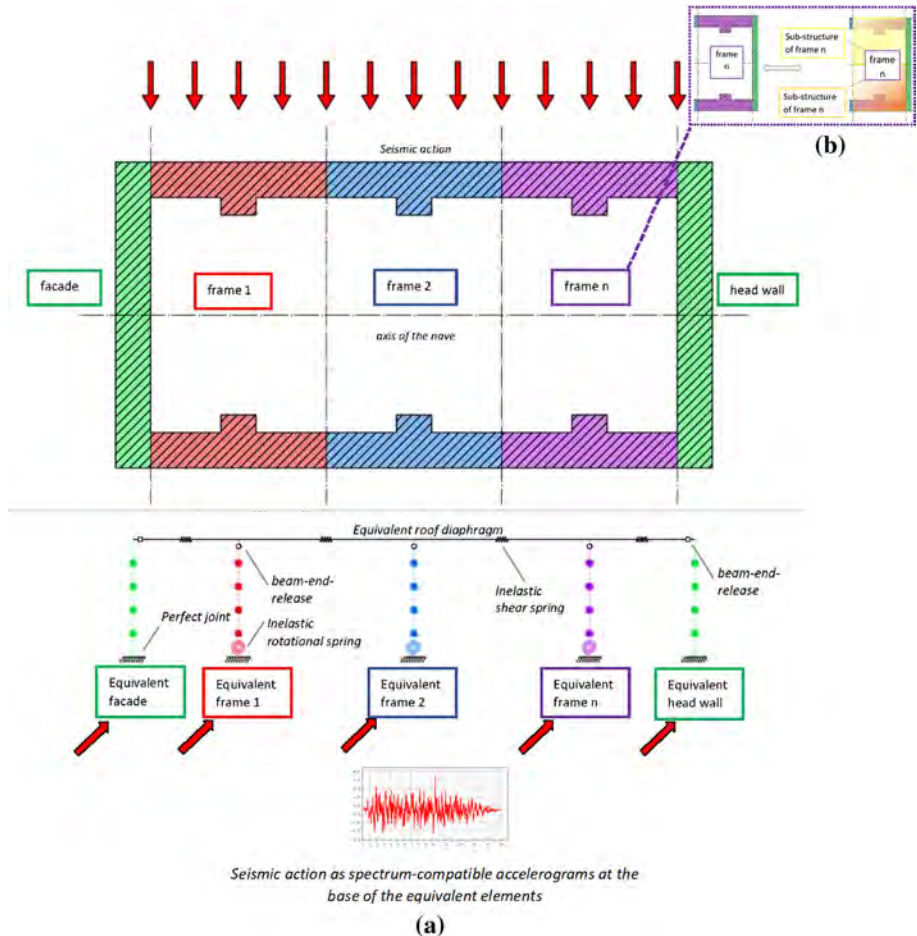
Fig. 1 a Example of seismic resistant frame identification for one nave configuration church (plan view) and related equivalent finite element model representation (longitudinal view): the façade and the head wall are identified in green; the seismic resistant frames are identified in red, blue and violet; the roof-diaphragm is identified in grey; b Identification (plan view) of the sub-structures characterizing the n -seismic resistant frame; the two sub-structures are identified respectively in yellow and orange
