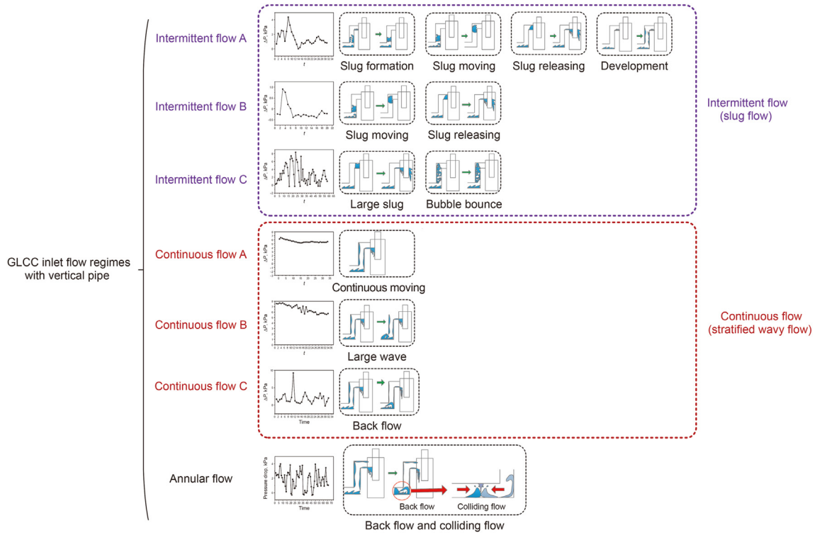
Fig. 5. GLCC flow regimes with vertical pipe.
