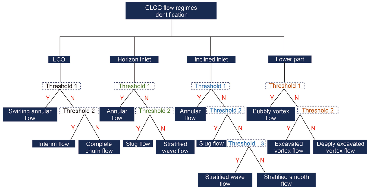
Fig. 12. Decision tree.
