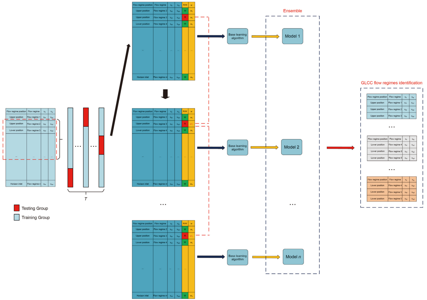
Fig. 10. Boosting algorithm.
