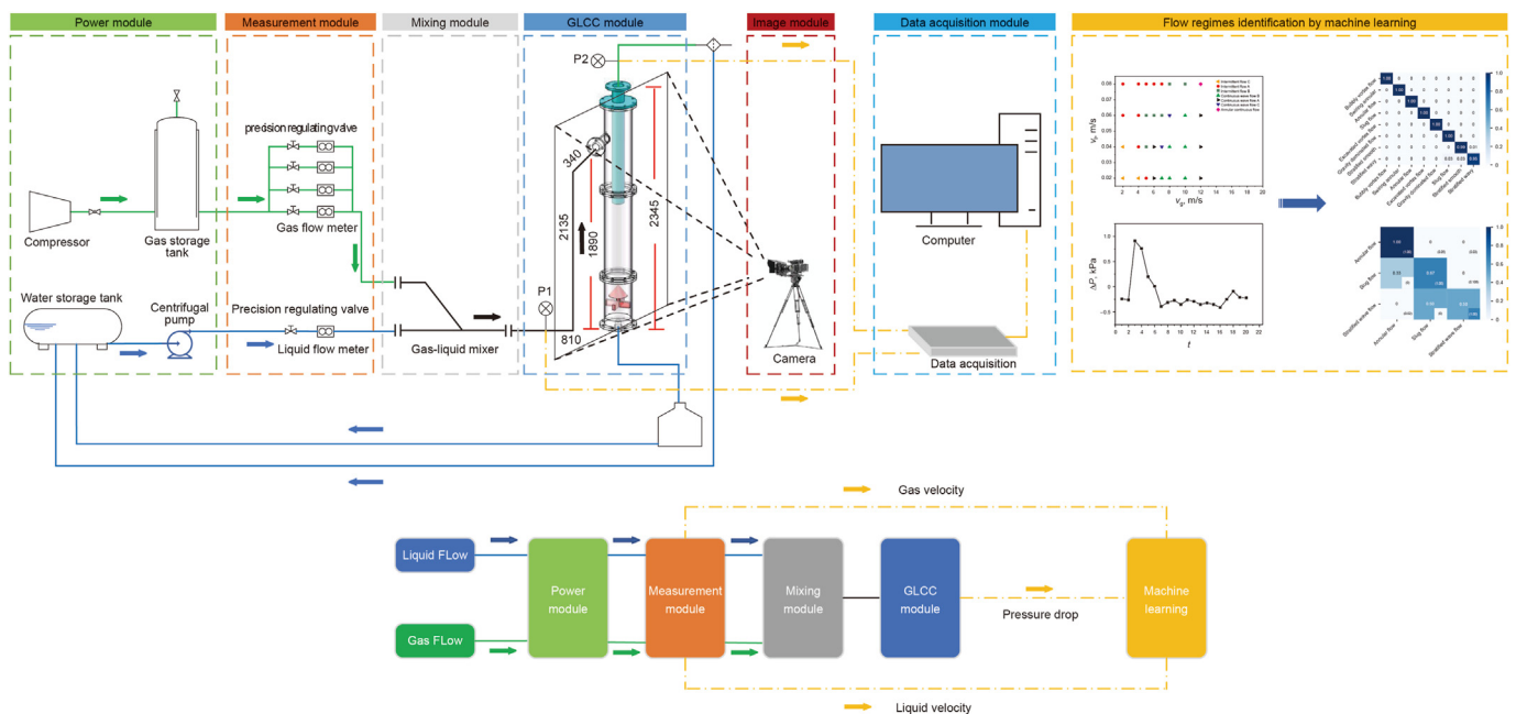
Fig. 3. Experimental setup.
