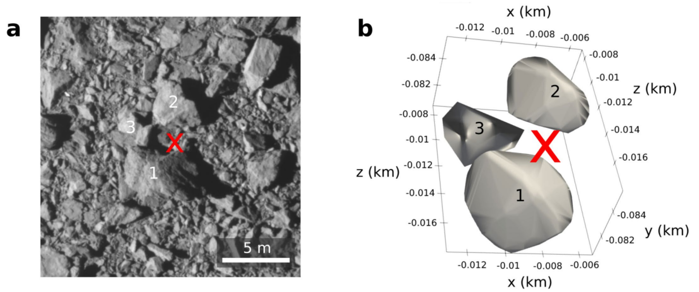
Extended Data Fig. 1 | Impact location. (a) Excerpt of the final full DRACO image of Dimorphos's surface ( dart_0401930049_43695_01_iofits ), -2 s before impact 1 . The red x indicates the approximate impact location. The north pole of Dimorphos is toward the top of the figure. (b) Convex hulls of the boulders at the impact location extracted from the impact site DTM 1 .
