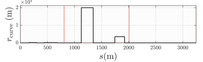
Fig. 5. Radius of the curves of the considered track
