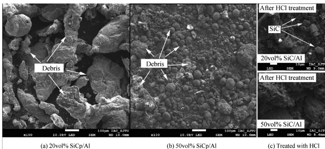
Fig. 11 Discharge debris of SiC p /Al composites.
