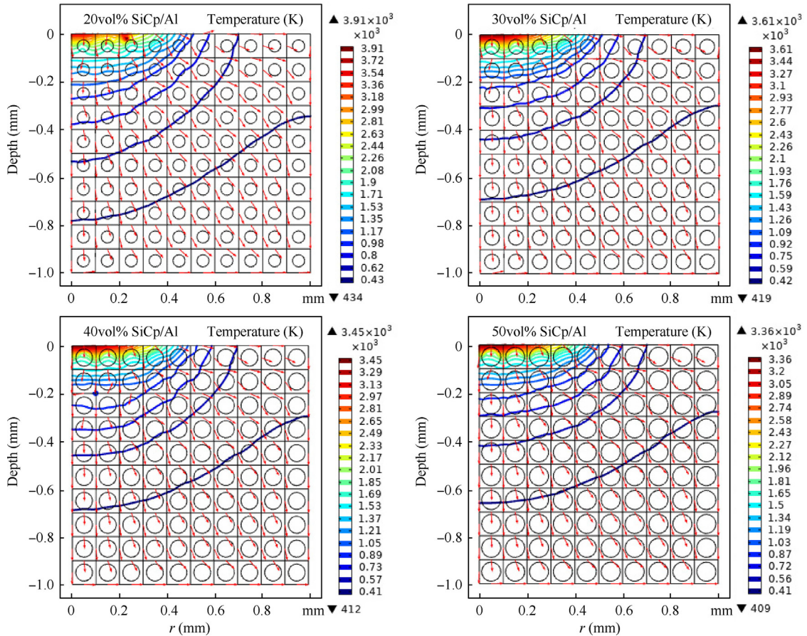
Fig. 5 Temperature distribution in \text{SiC}_p/\text{Al} composites ( t_{on} = 2 ms).
