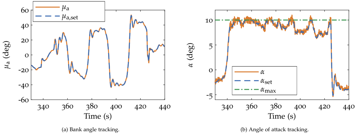
Figure 17: NDI control performance during one pumping cycle in turbulent wind condition (see Figure 10). Note that \alpha_{\max} represents a saturation limit on the angle of attack setpoint.
