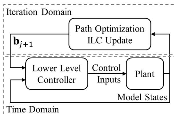
Figure 21: Basic block diagram for economic ILC, as applied to the optimization of the flight path (parameterized through the basis parameters \mathbf{b}_j ).
