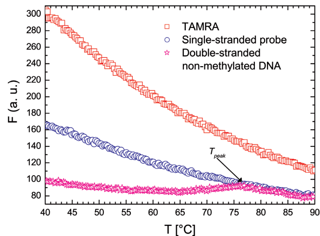
Figure 3. Steady-state fluorescence signal, F , measured as a function of temperature, T , for samples containing 50 nM concentrated free TAMRA (squares), TAMRA-labelled ss-DNA (circles) or TAMRA-labelled ds-DNA (stars, the probe was hybridized to target A), see Figure 1.
