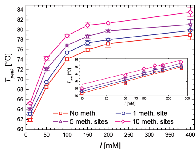
Figure 7. Values of T_{peak} , measured as a function of the ionic strength, I , for the duplexes formed by the dual-labelled probe with the non-methylated target oligonucleotide (a) of Figure 1 (squares), and with the target oligonucleotides (b), (e) and (i) of the same figure, containing one (circles), five (stars) and ten (diamonds) centrally located methylcytosine nucleotides, respectively. Inset: semi-logarithmic plot of the same data, together with their linear fits.
