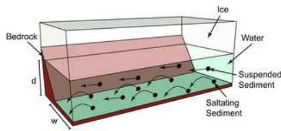
Fig 3. Illustration of a subglacial bedrock channel.
