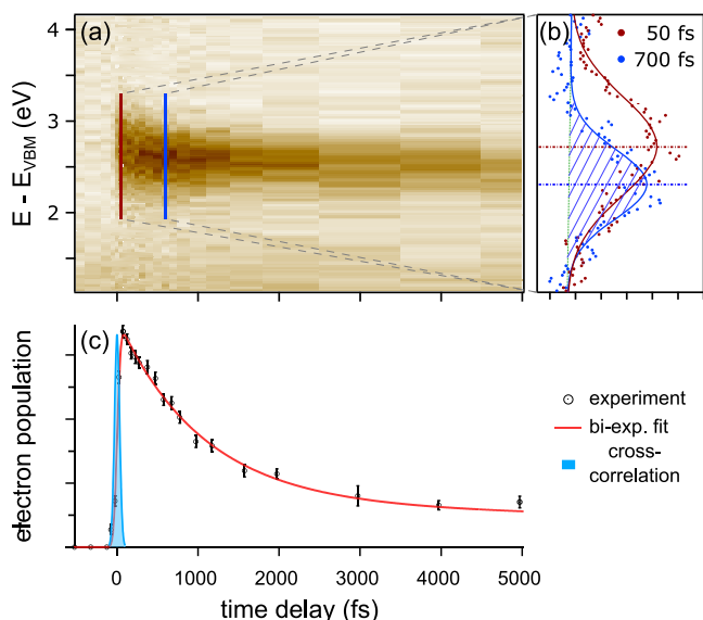
Figure 3. TR-ARPES data: (a) time evolution of the integrated photoemission intensity maps (the integration range is indicated by dashed lines in Figure 2b); (b) Gaussian fits of the integrated maps at the two time delays indicated by vertical lines in (a); (c) temporal dynamics of the CB population with a biexponential fit to the data. The time delay of 0 fs is fixed at the half-rise of the signal. The error bars indicate standard deviations of the Gaussian fit of the peak areas. The blue Gaussian represents the cross-correlation of the pump and probe pulses.
