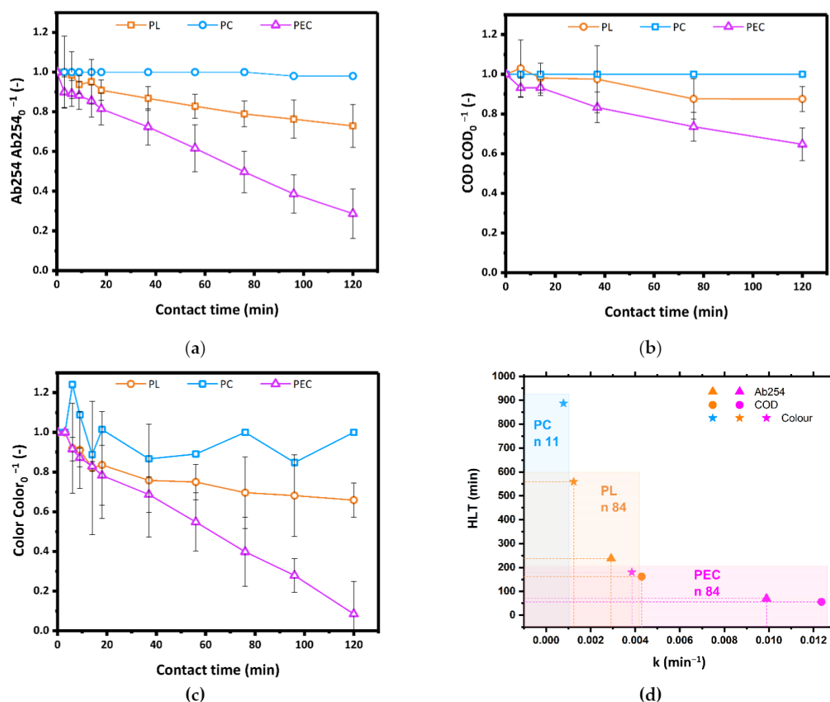
Figure 3. (a) Ab254, (b) COD and (c) residual color ( \text{Color} \cdot \text{Color}_0^{-1} ) relative to the corresponding parameters at t = 0 during PL, PC using 110 \text{ mg L}^{-1} \text{TiO}_2 powders and PEC using a \text{TiO}_2 photoanode. Confidence intervals have been calculated based on three repetitions. (d) Kinetic constants and HLT of PL and PEC for Ab254, COD and color removal; n: number of data (Source: author's own calculation/conception).
