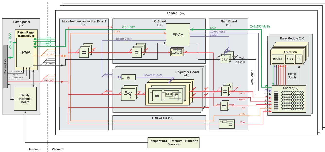
Fig. 8. Simplified block diagram of one DSSC camera quadrant. The green bold lines show the data path from the ASICs up to the EuXFEL DAQ back end. The total data rate delivered by all four quadrants is \sim 144 Gbit/s. Functional blocks required for the DEPFET operation are already implemented in the ASIC and tested, but are not shown in this diagram.
