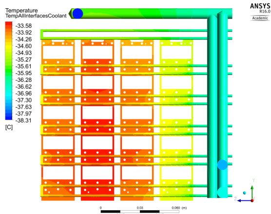
Fig. 10. Thermal situation at coolant path (horizontal lines) and interfaces of Cu cooling blocks to the module frames, based on hydrodynamic flow simulations of silicone oil coolant.
