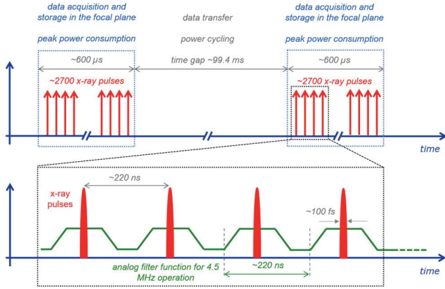
Fig. 1. Schematic representation of the EuXFEL X-ray delivery time structure. The FEL source delivers X-rays in pulse trains with a repetition rate of 10 Hz. Every pulse train consists of up to 2700 X-ray pulses with a temporal separation of 220 ns. The green trapezoidal shapes at the bottom represent the weighting function of the analog filter of the readout ASIC. For every train, 800 images can be stored in the memory of the ASICs. The data are then transferred to the EuXFEL DAQ during the \sim 99.4 -ms time gap between two consecutive pulse trains. Major parts of the chips are powered only during the bursts.
