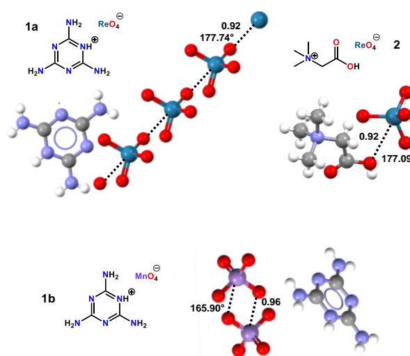
Figure 1 Ball and stick representation of the supramolecular polyanionic chain, dimer and cation-anion pair assembled by MaB in crystals of 1a (top left), 1b (bottom) and 2 (top right). For sake of clarity, structural formulas of the salts are reported and only one cation is depicted per structure. The normalized contacts (Nc) [18] and O–Mn/Re...O angles are given close to the MaB. Color code: whitish, hydrogen; grey, carbon; red, oxygen; blue, nitrogen; bluish, rhenium; violet, manganese.
