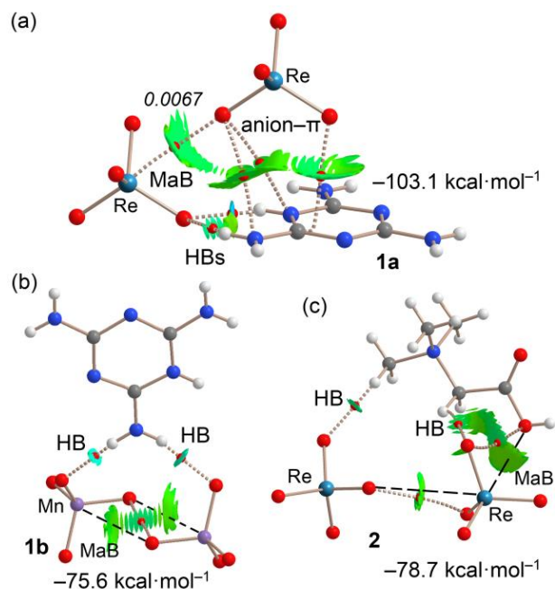
Figure 4 QTAIM distribution of intermolecular bond critical points (red spheres) and bond paths for the trimeric assemblies of compounds 1a (a), 1b (b) and 2 (c). The electron density at the bond CP that characterizes the MaB is given in italics (a.u.) The superimposed NCIplot isosurface (RDG isovalue = 0.5 a.u.) is shown, the cut-off \rho = 0.04 a.u. has been used. Color range -0.035 a.u. \leq (\text{sign}\lambda_2)\rho \leq 0.035 . Level of theory: PBE0-D3/def2-TZVP.
