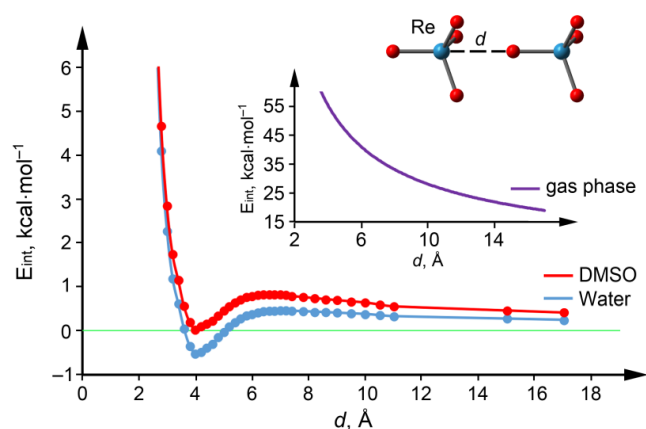
Figure 5 Energetic profiles obtained by varying the interatomic distance ( d ) in the ReO 4 - \cdots ReO 4 - dimer at the PBE0-D3/def2-TZVP level of theory.
