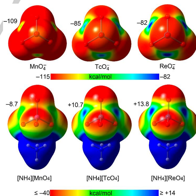
Figure 3 MEP surfaces of \text{MaO}_4^- (Ma = Mn, Tc and Re) anions and their ammonium salts at the PBE0-D3/def2-TZVP level of theory. The values at \sigma -holes are given in \text{kcal mol}^{-1} .
