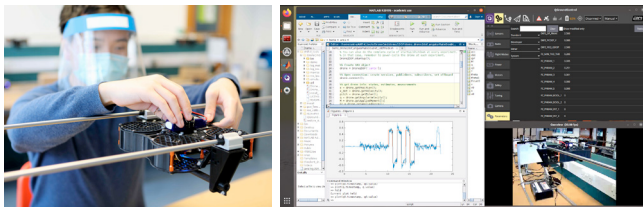
Fig. 10. Demonstration of the hybrid-mode lab. Left: battery replacement by an on-site TA. Right: controller tuning (the upper-right window), experimental data collection (the left window), and real-time UAV monitoring (the lower-right window) by students via remote access
