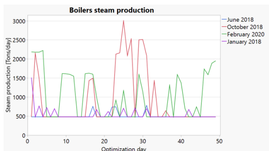
Fig. 7. Steam produced by the boilers in the different periods
