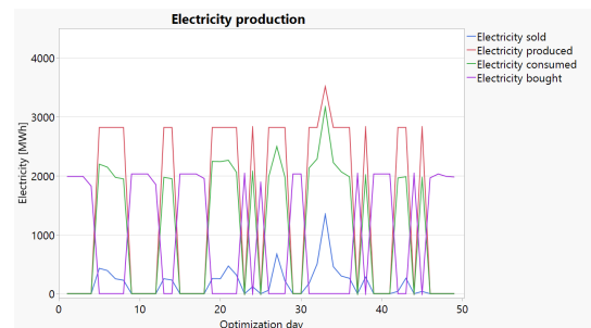
Fig. 6. Electricity produced and sold in Period 4.
