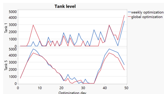
Fig. 8. Tank 1 and 5 level for June 2018 optimization.
