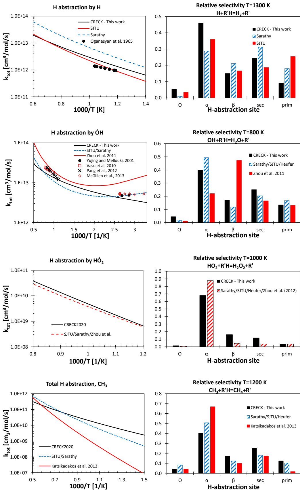
Figure 7. (Left) Total rate constants of H-atom abstraction reactions by \dot{\text{H}} , \dot{\text{OH}} , \dot{\text{HO}}_2 , and \dot{\text{C}}\text{H}_3 on n -butanol from this work (black) and from the literature. 5,41–45,48,49,83,87 (Right) Relative selectivity to the different H-atom abstraction site for n -butanol from this work (black) and from the literature.
