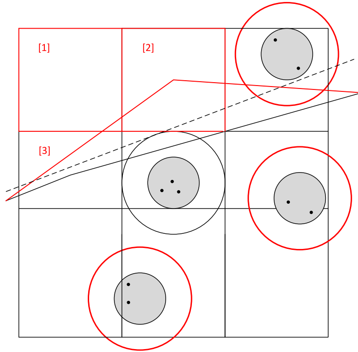
Figure 7: Example of critical cluster: the solid edge e , generated at a given stage of the TSR algorithm, passes through a cluster without passing through its kernel. The dashed line represents the original segment for the edge e . The red line represents the result of the application of the REROUTE() procedure to edge e : since there are no useful clusters, then case (b2) occurs. Procedure FREE-CELLS() returns cells 1, 2 and 3: cell 3 is not useful for re-routing e outside the cluster, while between cell 1 and 2, the last one is chosen because it produces a smaller distance from e.os .
