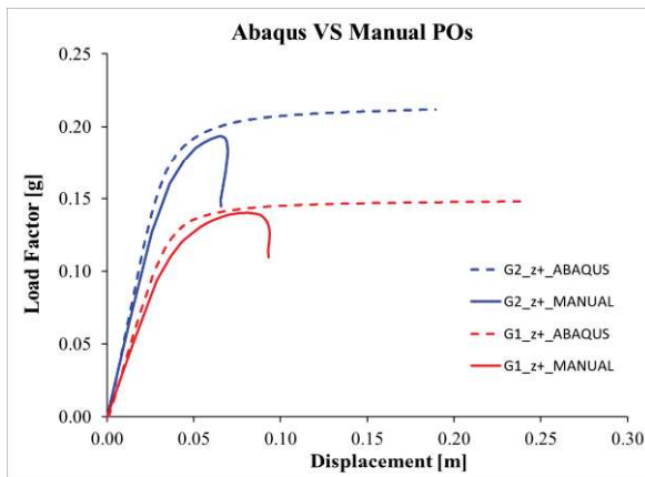
Figure 7 Abaqus vs Manual POs: original model.
