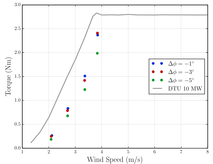
Fig. 26. Wind tunnel test results, for \lambda_V = 3 : torque.
