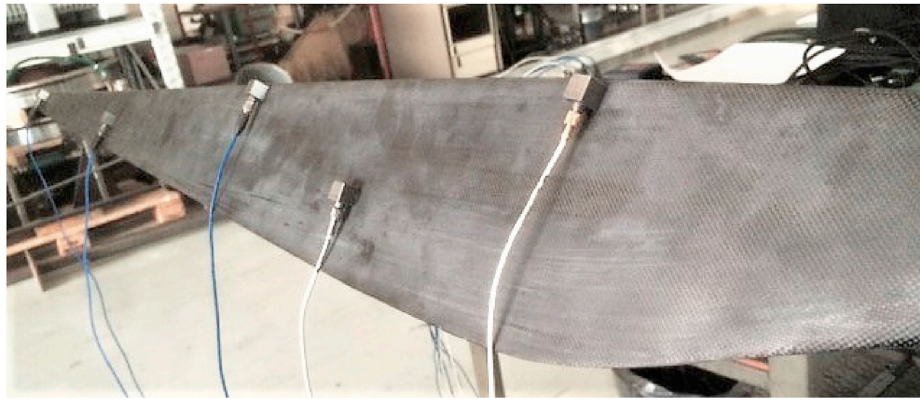
Fig. 20. Experimental setup.
