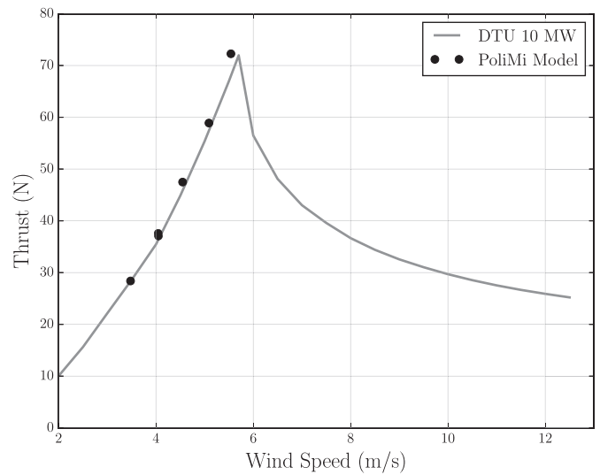
Fig. 23. Wind tunnel test results compared with the reference scaled DTU 10 MW performance: thrust.
