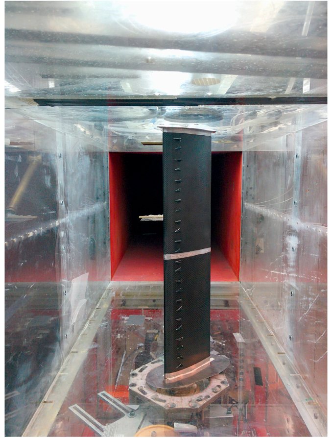
Fig. 4. DTU red wind tunnel test section.
