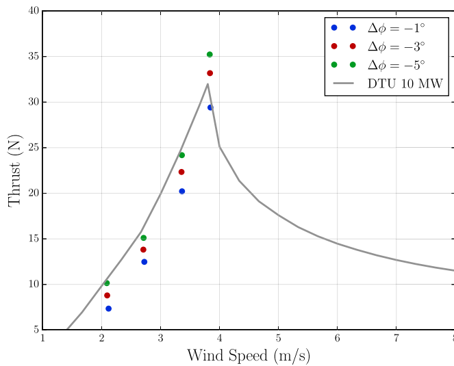
Fig. 25. Wind tunnel test results, for \lambda_V = 3 : thrust.
