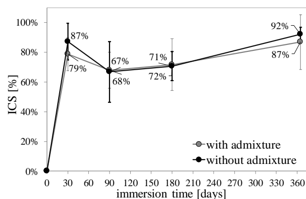
Figure 15. Index of crack sealing for thin beam specimens tested in 4-point bending.
