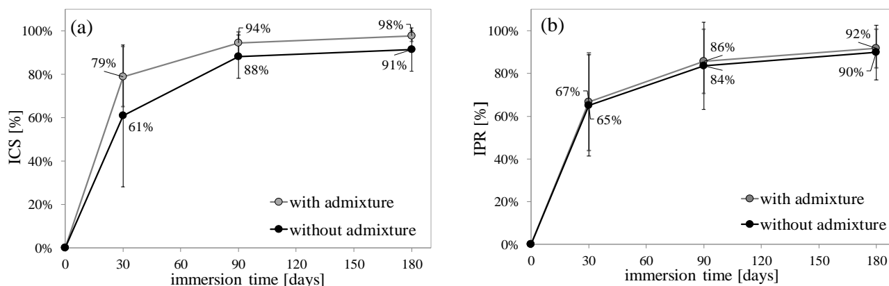
Figure 12. Index of crack sealing (a) and of permeability recovery (b) for split-cracked disks undergoing up to six months permanent immersion in tap water.
