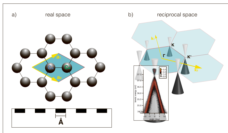
Fig. 1. (a) Real space sketch of graphene. The unit cell (central rhomb) contains two carbon atoms C_A and C_B , one from each sublattice. (b) Corresponding reciprocal space picture with the first Brillouin zone (BZ) in the center. The electronic band structure around E_F consists of six double cones touching at the K and K' points of the BZ. ARPES measurement of a p-doped graphene sample showing a branch of one of the Dirac cones.
