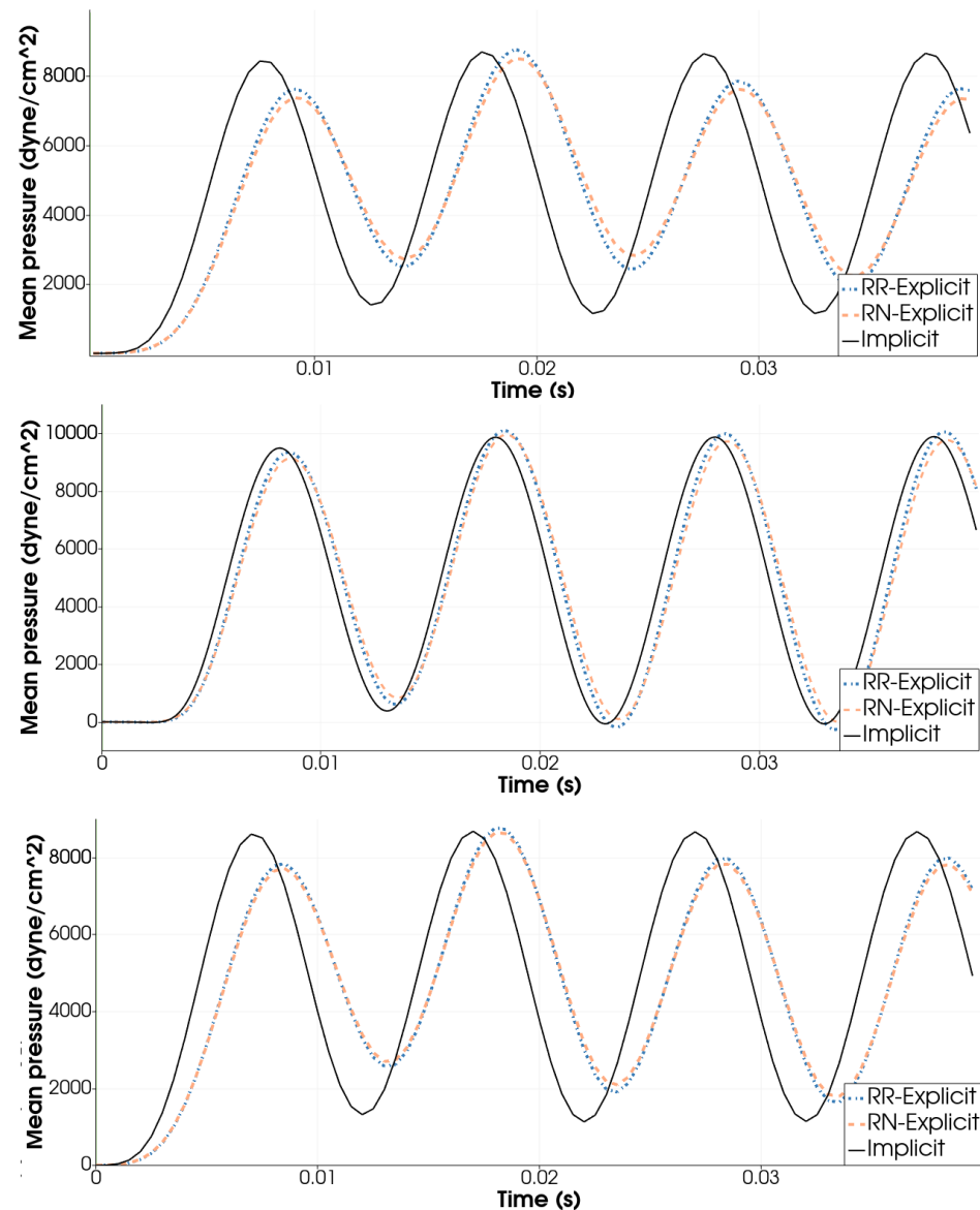
Figure 2. Mean pressure at section z = 2.5 cm for \hat{P} = 5000 : \Delta t = 0.0005 s, \gamma_{ST} = 1.5 \times 10^5 ( top ), \Delta t = 0.000125 s, \gamma_{ST} = 1.5 \times 10^5 ( middle ), and \Delta t = 0.0005 s, \gamma_{ST} = 3 \times 10^5 ( bottom ). Test I.
