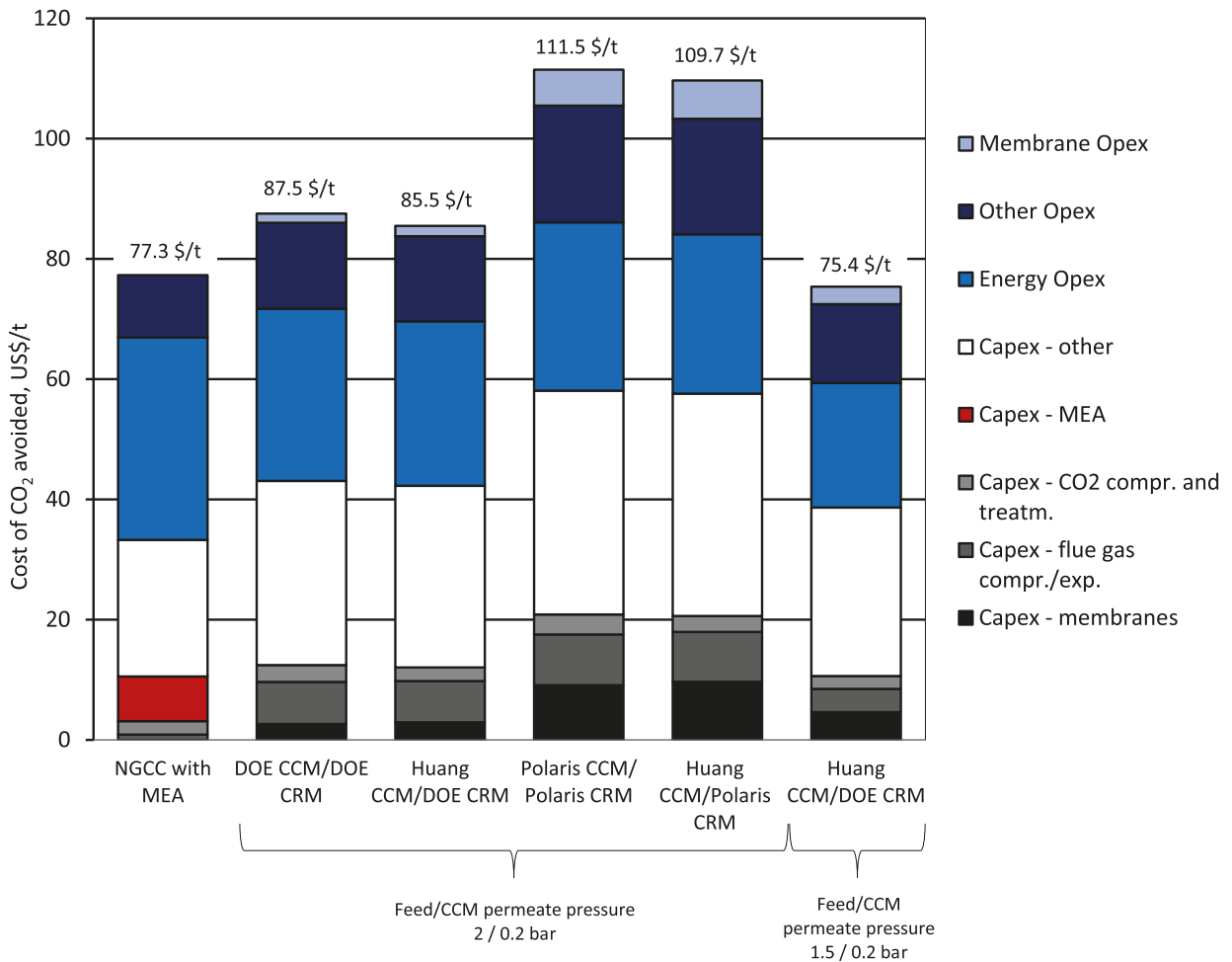
Fig. 9. Effect of membrane type on the cost of CO 2 avoided.
