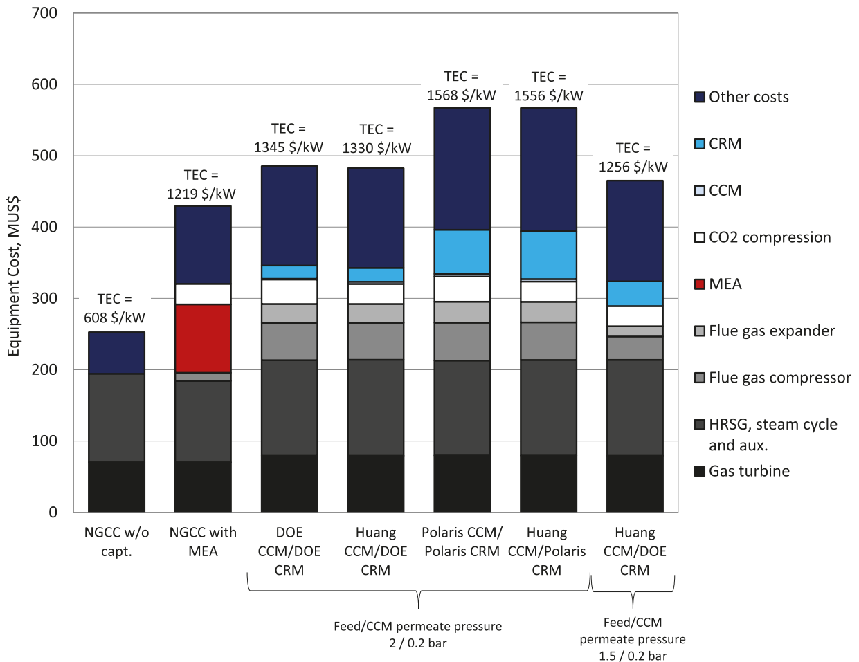
Fig. 7. Breakdown of the equipment costs and total specific equipment cost.
