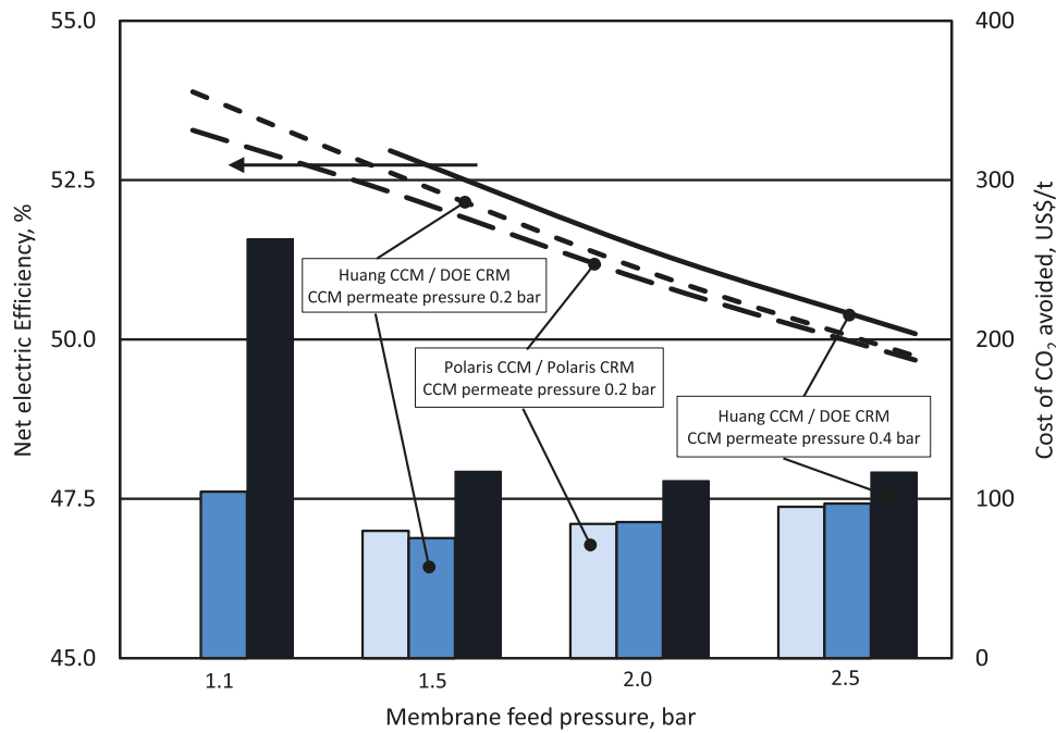
Fig. 10. Cost of CO 2 avoided and electric efficiency vs. membrane feed pressure for different CCM permeate pressures.
