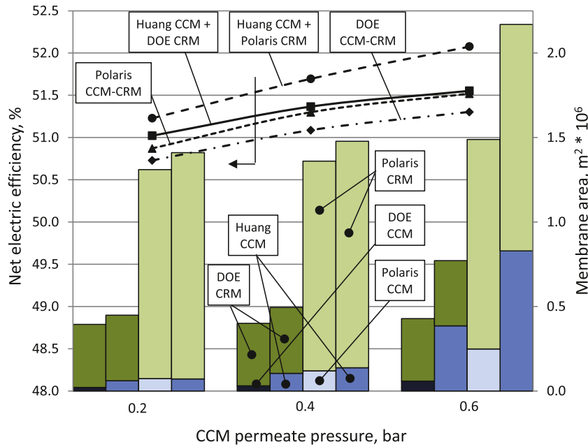
Fig. 5. Effect of CCM permeate pressure on efficiency and membrane surface area for cases with 2 bar of feed pressure.
