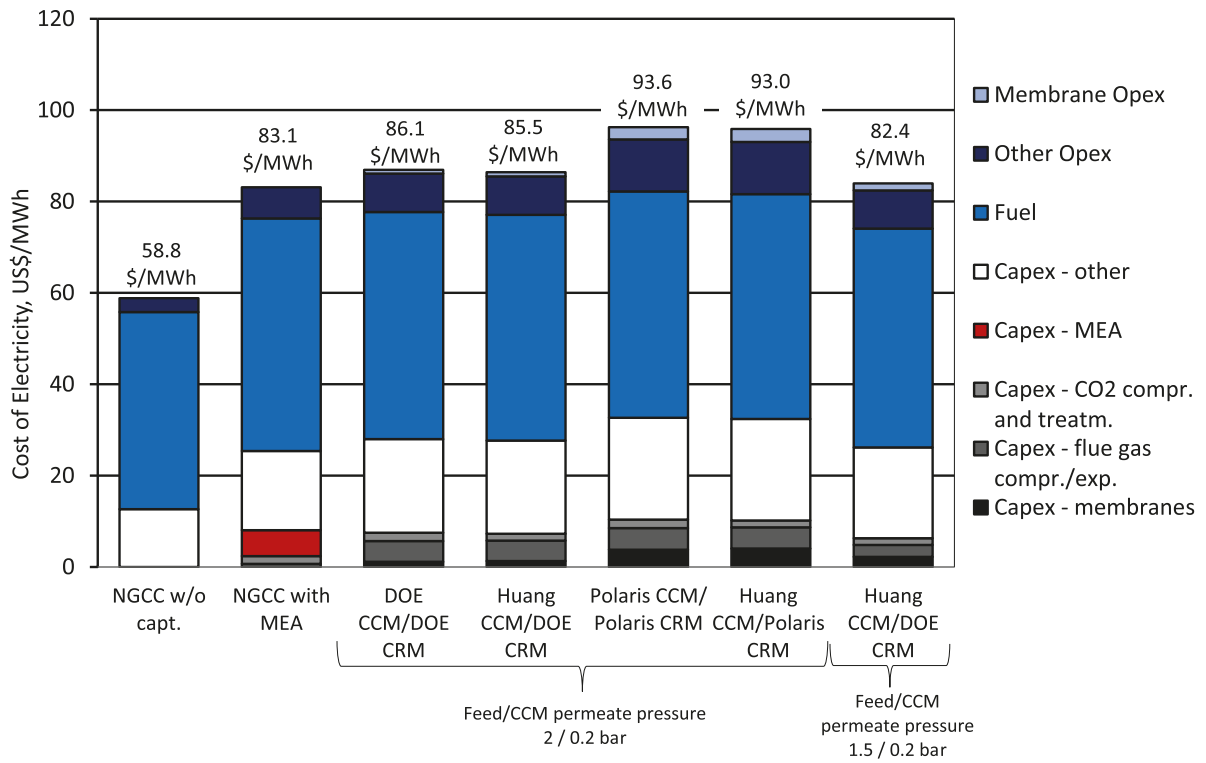
Fig. 8. Breakdown of the cost of electricity.
