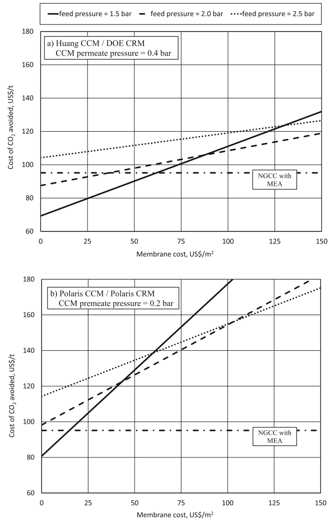
Fig. 13. Cost of CO 2 avoided with variations in the specific membrane cost for different feed pressures and a price of electricity of 90 €/MWh.
