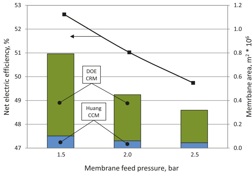
Fig. 6. Effect of membrane feed pressure on efficiency and membrane area for the Huang/DOE case, with CCM permeate pressure of 0.2 bar.
