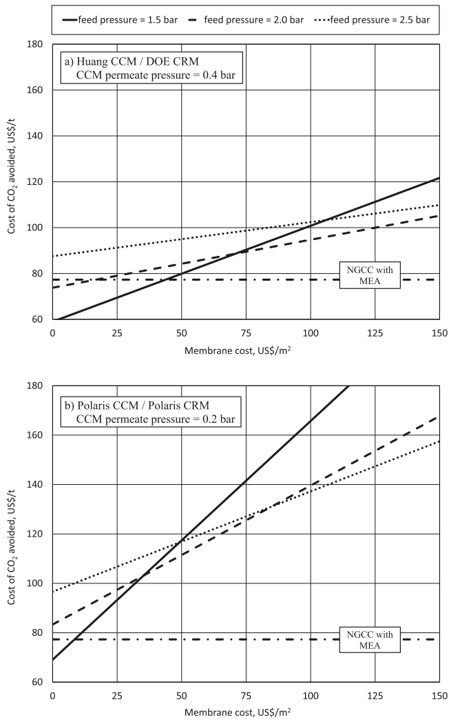
Fig. 12. Cost of CO 2 avoided with variations in the specific membrane cost for different feed pressures and a reference price of electricity (58.8 $/MWh).
