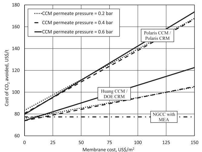
Fig. 11. Cost of CO 2 avoided at different membrane costs for different membranes and CCM permeate pressures, for membrane feed pressure of 2 bar.
