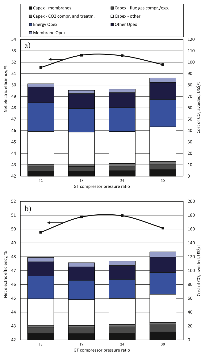
Fig. 14. Cost of CO 2 avoided and plant efficiency vs. gas turbine pressure ratio for the Huang CCM/DOE CRM case with feed and CCM permeate pressures of 1.5 and 0.2 bar (a) and the Polaris/Polaris case with feed and CCM permeate pressures of 2 and 0.2 bar (b).
