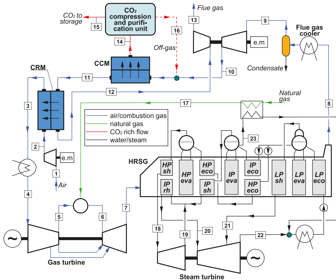
Fig. 1. Process configuration of the NGCC power plant with CO 2 membranes assessed in this work.
