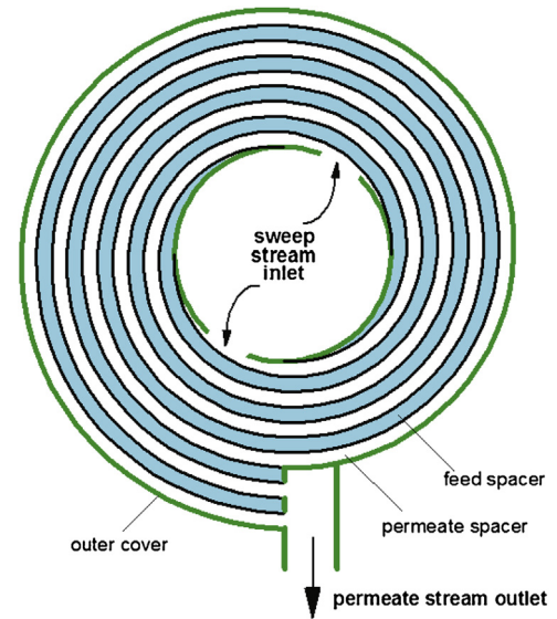
Fig. 2. Cross section of the 4-port spiral wound module considered in the paper. In this sketch, four membranes sheets are wound around the central distribution pipe.
