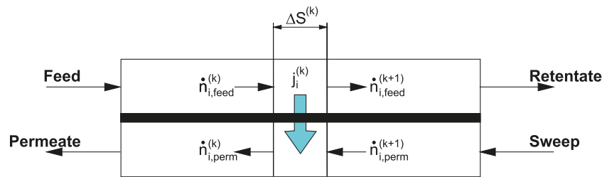
Fig. 4. Axial discretization of the membrane module.
