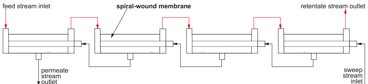
Fig. 3. String of 4-port modules connected in series in counter-current configuration.
