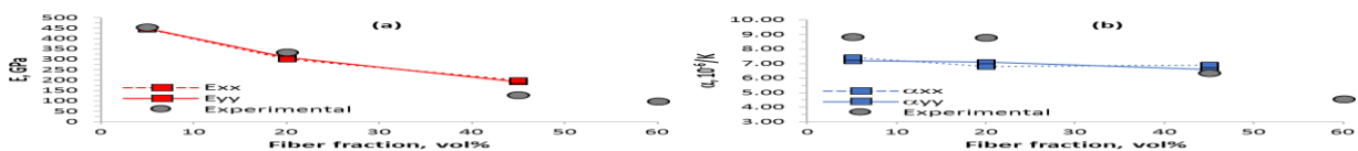
Fig. 7: Plots of homogenized a) Young's modulus, E , and b) coefficient of thermal expansion, \alpha , of reinforced composites obtained by 2D route compared to experimental values (grey circles).
