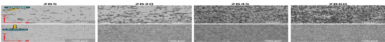
Fig. 4: SEM images of the materials containing 5, 20, 45 and 60 vol% fibres showing examples of transverse (upper images) and perpendicular (lower images) section views.
