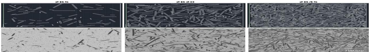
Fig. 6: (upper images) Numerically generated microstructure of the materials containing 5, 20 and 45 vol% fibres with corresponding SEM images (lower images). All images have the same magnification.
