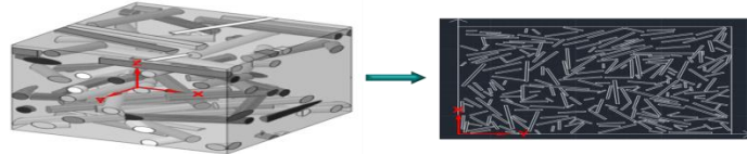
Fig. 2: Numerical representation of a 3D microstructure where 20 vol% short fibres are aligned along the X-Y plane (left) and simplified in a 2D representation (right).
