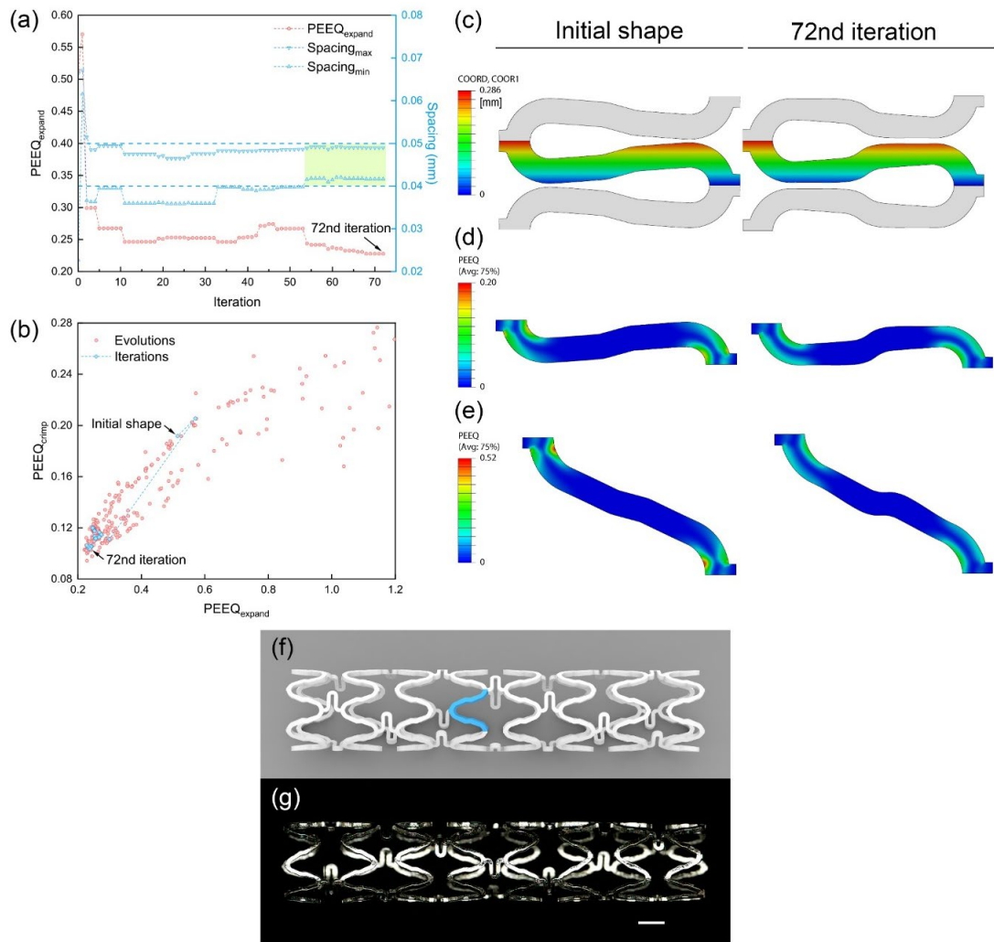
Figure 3. Shape optimization based on 2D strut model. (a) Optimization history of the maximum equivalent plastic strain after expanding ( PEEQ_{expand} ) and range of spacing between adjacent strut edges after crimping ( Spacing_{max} and Spacing_{min} ). The results matching the boundary conditions of spacing were shaded for distinction. (b) PEEQ_{crimp} versus PEEQ_{expand} plots of attempt evolutions and selected output of each iterations. (c) The strut coordinates in compress direction for initial and optimized shape. (d, e) The distributions of PEEQ for initial and optimized shapes after crimping and expanding. (f, g) The 3D model and the manufactured optimized stent (scale bar represents 1 mm).
