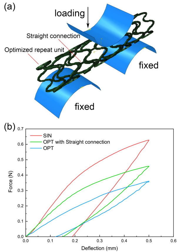
Figure S2. Three-point bending test. (a) The finite element assembly of three-point bending simulation. In addition to SIN and OPT stents, a stent composed with optimized repeat unit and straight connection was built for flexibility test. The span length between two static supports is 10.0 mm and the deflection of load applicator is 0.5 mm based on the ASTM F2606 standard. (b) The curves of force and deflection for 3 stents. Optimized repeat units improve the flexibility of the stent. Moreover, ‘n’ shape links make the OPT stent more compliancy.
