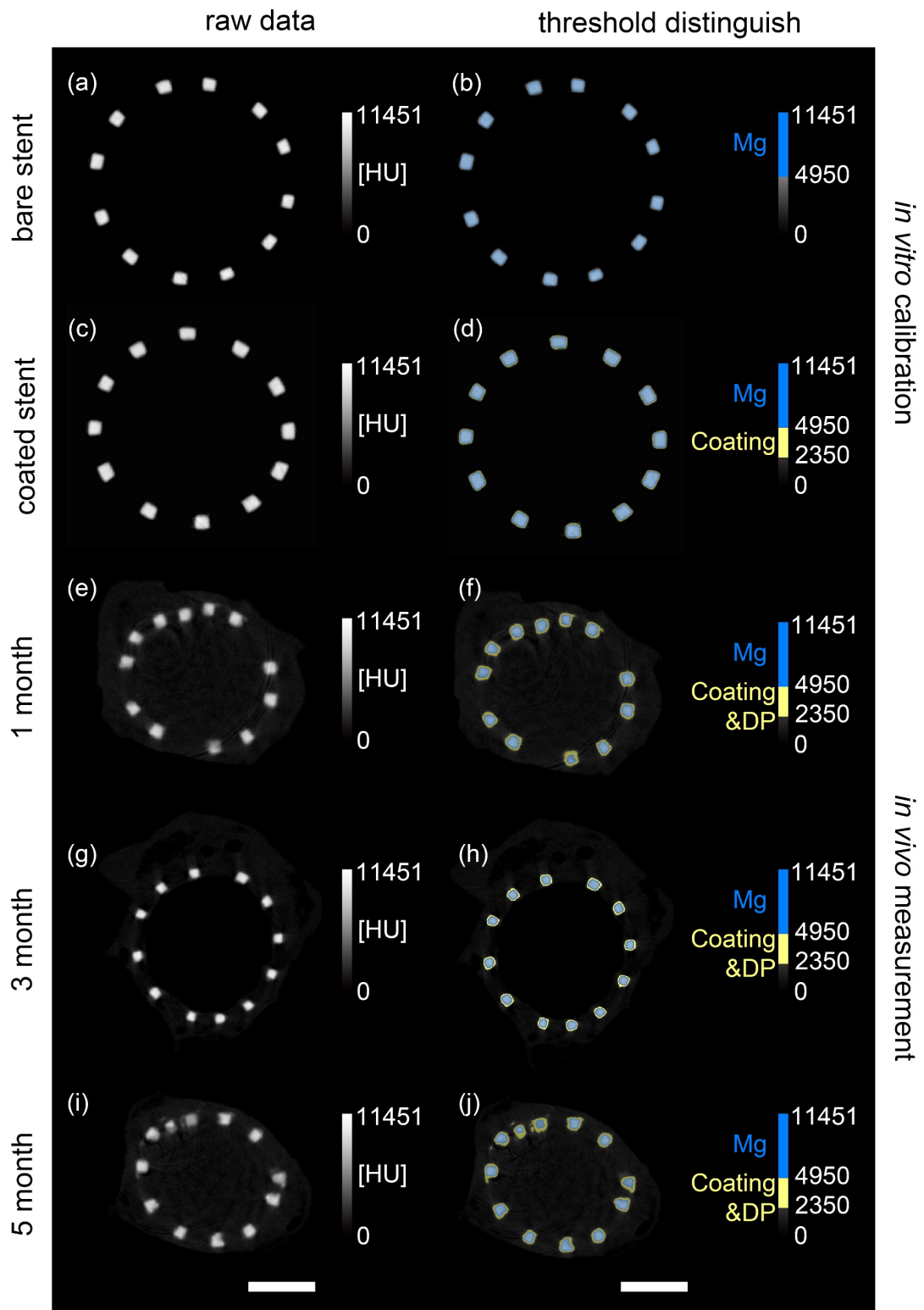
Figure S4. The threshold distinguishing and calibration of Mg stent cross-sections by Micro-CT. The left panel (a, c, e, g, i) shows the reconstructed section of micro-CT raw data. The range of threshold is from 0 to 11451 Hounsfield unit (HU). Bare stents and coated stents before implantation were used to calibration the threshold for Mg strut and polymer coating based on the volume measured by the Archimedean method in vitro . (b) The threshold of Mg strut is [4950, 11451] HU and (d) the threshold
