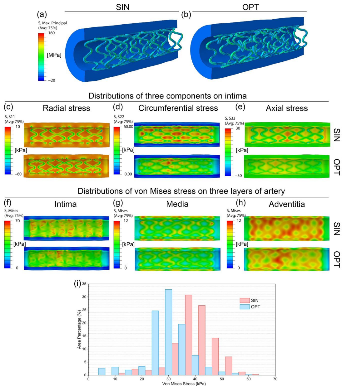
Figure 7. Result of stents implantation in the vascular vessels. (a, b) Distributions of the maximum principal stress of the SIN and OPT stents. (c, d, e) Distributions of radial, circumferential and axial stress components in the stented region of the intima layer for the SIN (top) and OPT (bottom) stents. (f, g, h) Distributions of von Mises stress in the intima, media and adventitia layers for the SIN (top) and OPT (bottom) stents. (i) The histogram shows the area distribution of von Mises stress on the surfaces of the intima in the stented region for the SIN and OPT stents. The range of each bin is 5 MPa. Compared to the SIN stent, a significant reduction could be found in relative high-stress regions ( \geq 40 kPa) of the OPT stent.
