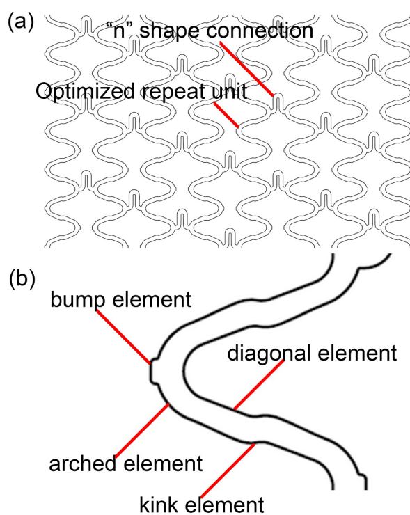
Figure S1. The structure of the optimized stent. (a) The CAD drawing for laser cutting and (b) the design of repeat unit consists of bump element, arched element, diagonal element and kink element.
