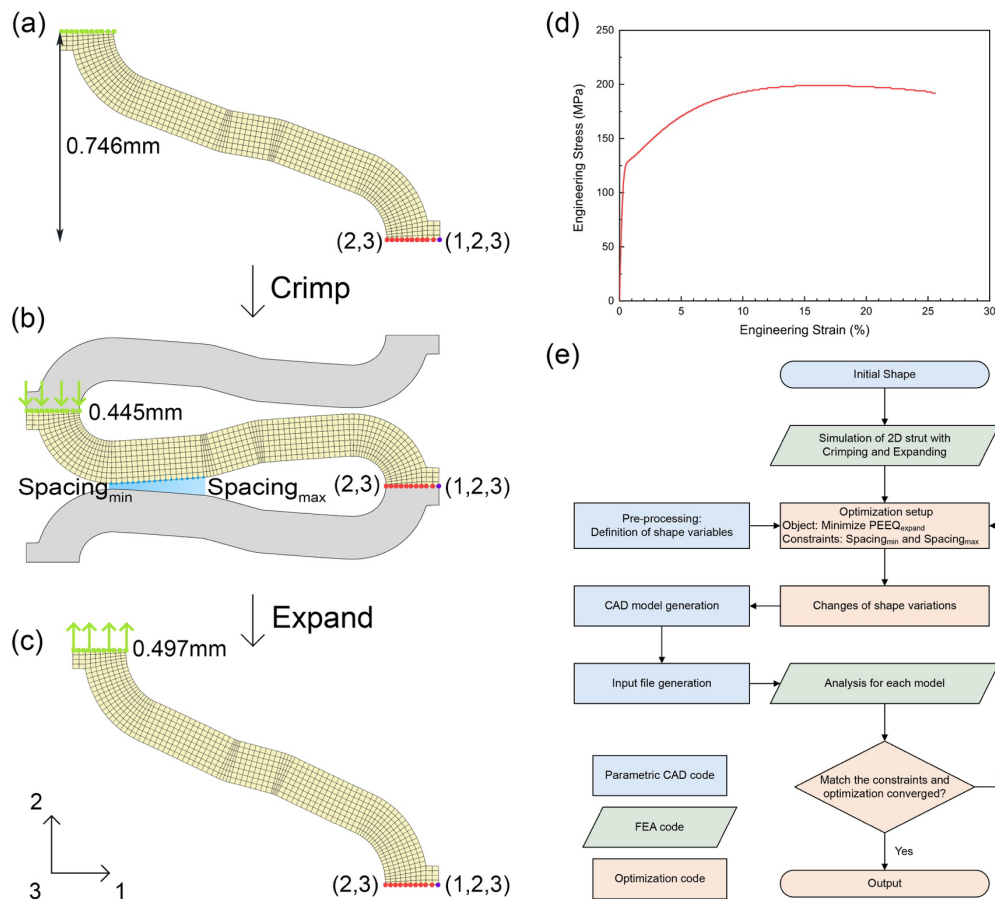
Figure 2. The boundary conditions and displacement loadings for the 2D strut model during shape morphing program. (a) The 2D initial shape (b) the crimped status and (c) the expanded status. The spacing values were introduced to modify the shape of the adjacent borders of the crimped strut. (d) The engineering stress-strain curve of JDBM used for manufacturing the cardiovascular stents. (e) The flow chart of the shape optimization procedure for the 2D strut model.
