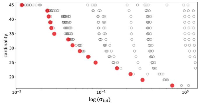
Fig. 5. Search space of the sequential approach.
