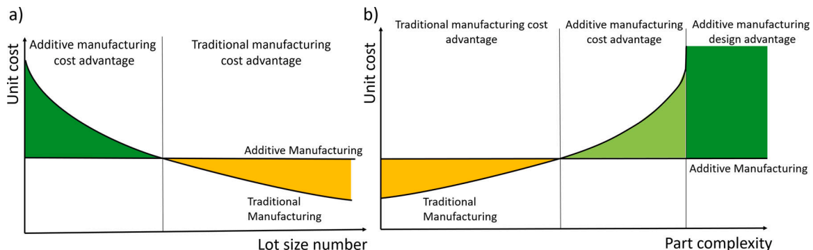
Fig. 4. Unit cost for additive and traditional manufactured parts referred to a) production volume and b) complexity or customization of the parts and influence of new design opportunities by additive manufacturing on unit cost referred to complexity of the parts compared to traditional processes. The green area shows the more favorable range for AM as manufacturing method.
