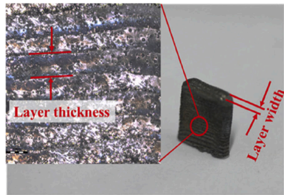
Fig. 10. Thin wall structure with marked layer thickness and width made from YSZ by Fan et al. [103].
