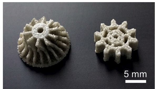
Fig. 6. Complex structure made from iron oxide doped aluminum oxide powders by a nano-second pulsed green Nd-YAG laser.
