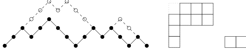
Figure 1: A pair of Dyck paths \gamma (thick) and \gamma' (dashed), with \gamma < \gamma' , and the corresponding set of skew Ferrers shapes.
