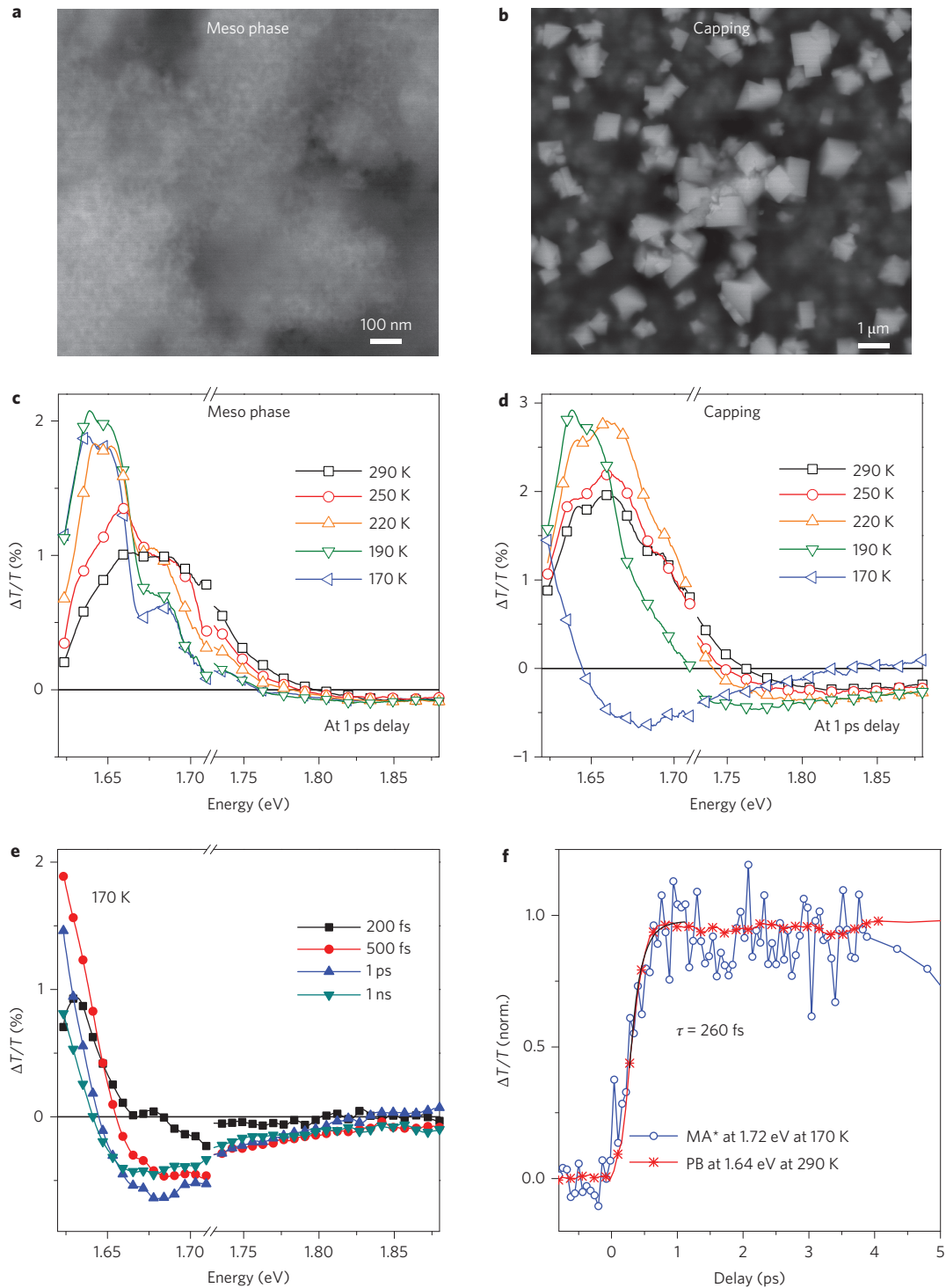
Figure 1 | Temperature-dependent transient absorption spectra of MAPbI 3 meso phase and capping layer. a,b , SEM images of the meso phase (a) and capping layer (b) of the 3- \mu m-thick MAPbI 3 sample. c , Temperature dependence of the TA spectra at 1 ps pump-probe delay of the meso phase. d , Temperature dependence of the TA spectra at 1 ps pump-probe delay of the capping layer. e , TA spectra between 200 fs and 1 ns at 170 K for the capping layer. f , Dynamics probed at 1.72 eV (MA* band) for the capping layer at 170 K compared to the dynamics probed at 1.64 eV (PB band) of the same sample at room temperature (290 K). For all TA measurements, the excitation wavelength was at 2.38 eV with an excitation density of \sim 5 \times 10^{17} \text{ cm}^{-3} .
