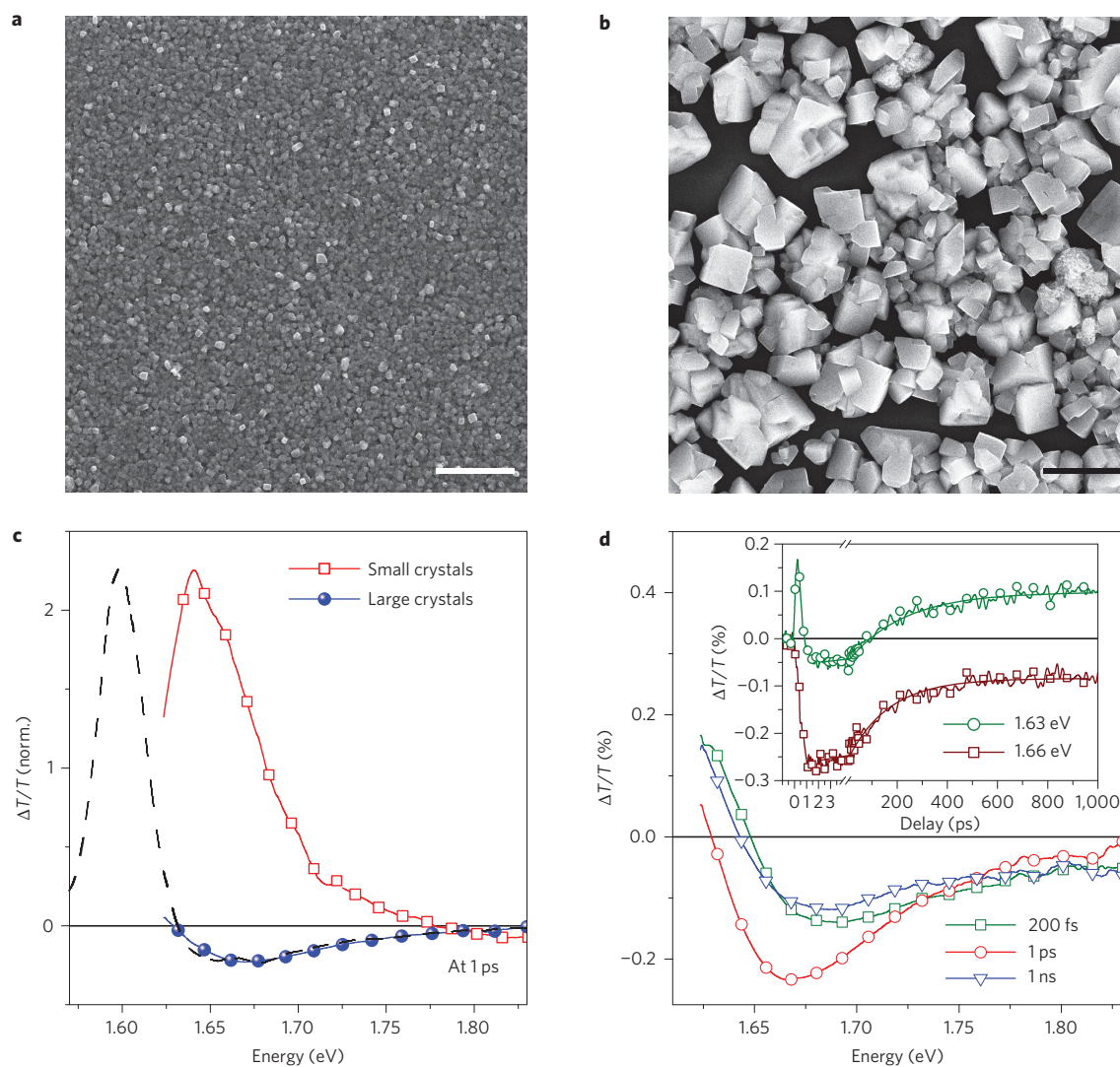
Figure 2 | Photo-induced excited population of MAPbI 3 as a function of crystal size. a,b , SEM images of perovskite films with average crystal dimensions of <200 nm ( a ) and \sim 1\ \mu\text{m} ( b ). Scale bars, 2 \mu\text{m} . c , TA spectra at room temperature, at 1 ps pump-probe delay, of the two samples shown in a and b (red squares and blue circles, respectively) as well as the TA spectrum (dashed line) of the sample in b , taken at 77 K, redshifted by 95 meV. d , TA spectra at different time delays, at room temperature, from the sample shown in b . Inset: dynamics probed at 1.63 eV and 1.66 eV. For all TA measurements, the excitation wavelength is at 2.38 eV with an excitation density of \sim 5 \times 10^{17}\ \text{cm}^{-3} .
