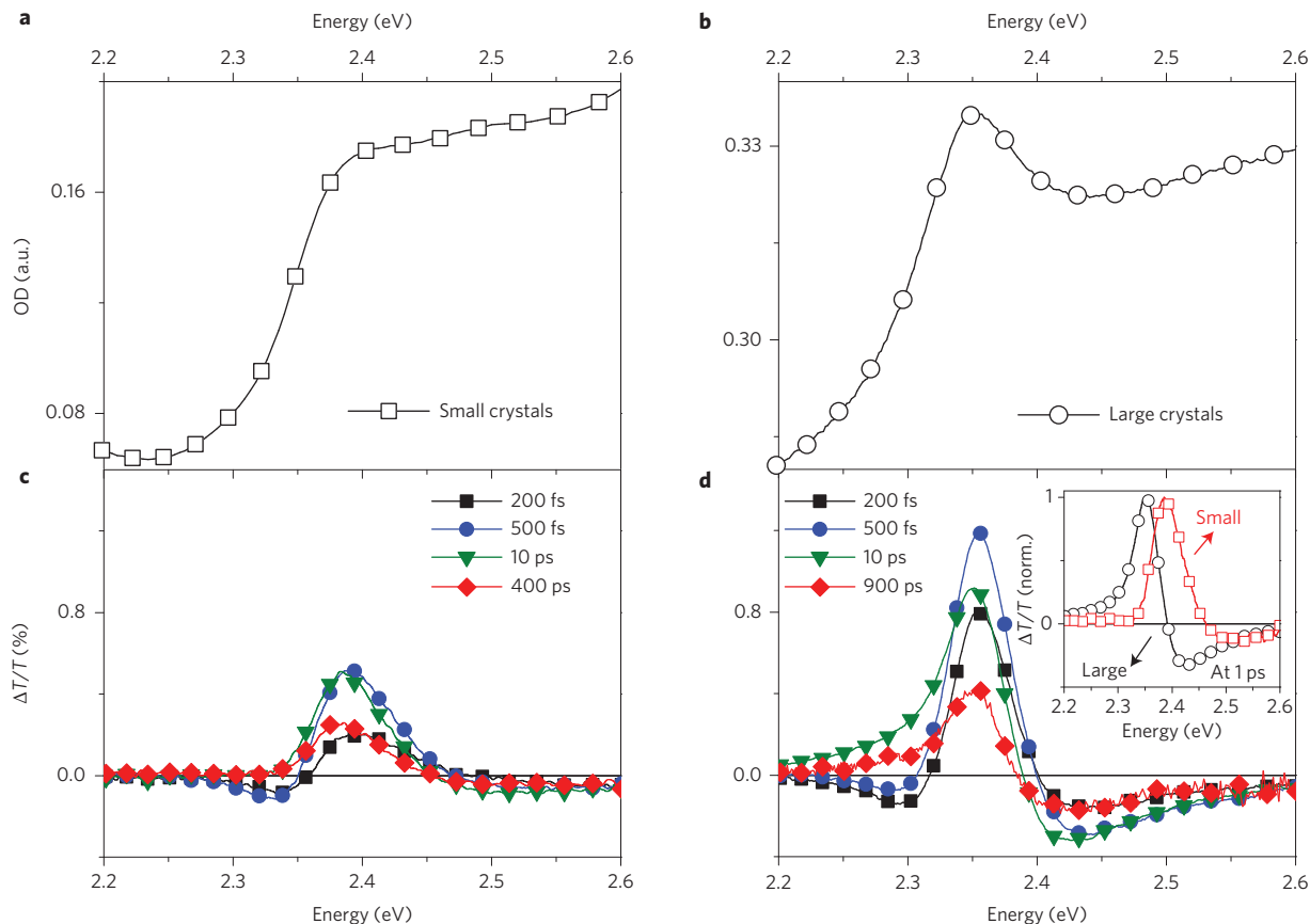
Figure 3 | Photo-induced excited population of MAPbBr 3 as a function of crystal size. UV-vis absorption spectra from MAPbBr 3 films with average crystallite dimension of \ll 100\text{ nm} (a) and \sim 1\text{ }\mu\text{m} (b). c,d. TA spectra at different time delays, at room temperature, from samples with small (c) and large (d) crystallites (for SEM images see Supplementary Fig. 12). Inset (d): comparison of TA spectra at 1 ps of small and large MAPbBr 3 crystals. For all TA measurements, the excitation wavelength is at 3.1 eV with an excitation density of \sim 1 \times 10^{17}\text{ cm}^{-3} .
