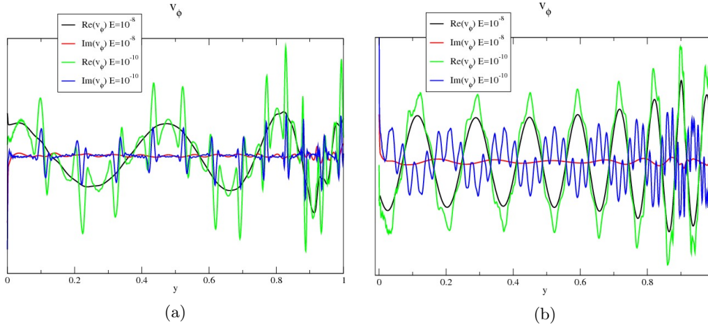
Figure 15: Profile of v_\phi for mode tagged “1” in fig. 8 (a) and mode 6 (b). The profile is shown along the radial direction starting from inner critical latitude. Note the smoothness of the black lines ( E = 10^{-8} ) and the emergence of small-scales in the green lines ( E = 10^{-10} ).
