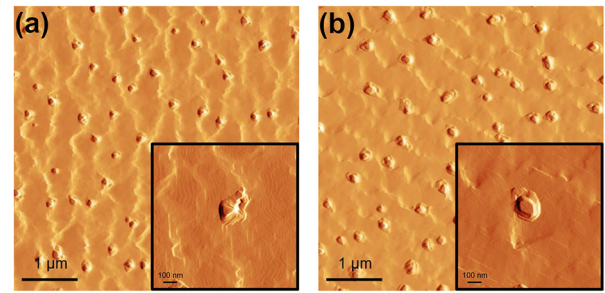
FIG. 2. (a) 5 \times 5 \mu\text{m}^2 AFM tapping amplitude image of sample D (the inset shows a 1 \times 1 \mu\text{m}^2 AFM tapping amplitude image of an individual QD with a triangular pyramidal shape); (b) 5 \times 5 \mu\text{m}^2 AFM tapping amplitude image of sample E (the inset shows the 1 \times 1 \mu\text{m}^2 AFM tapping amplitude image of an individual QD with an asymmetrical hexagonal-like pyramidal shape).
