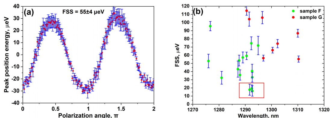
FIG. 4. (a) Polarization dependence of the QD emission line (1310 nm) of sample G with a finite FSS of 55 \pm 4 \mu\text{eV} . (b) Statistical distribution of FSS of samples F (green points) and G (red points).
