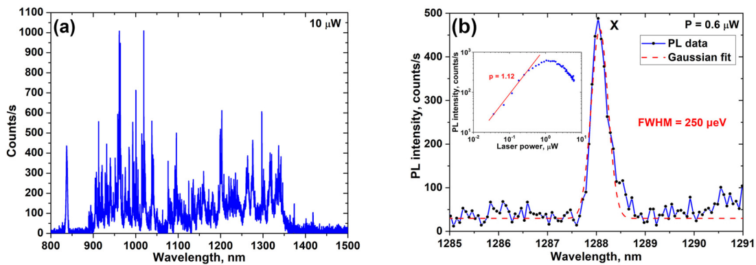
FIG. 3. (a) The broadband PL spectrum of sample F with a cw excitation of 10 \mu\text{W} ; (b) the luminescence spectrum of an individual InAs QD of sample F with a cw excitation of 0.6 \mu\text{W} . The inset shows the power dependence of PL intensity of the observed neutral X line.
