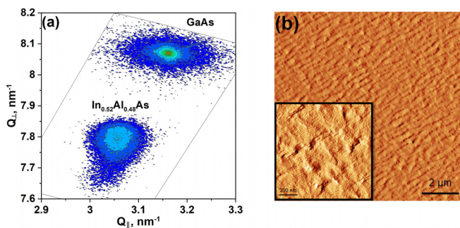
FIG. 1. (a) XRD reciprocal space map, taken around the (224) asymmetric Bragg reflection of sample A. (b) 10 \times 10 \mu\text{m}^2 AFM tapping amplitude image of sample C (the inset shows the 1 \times 1 \mu\text{m}^2 AFM tapping amplitude image of the sample).
