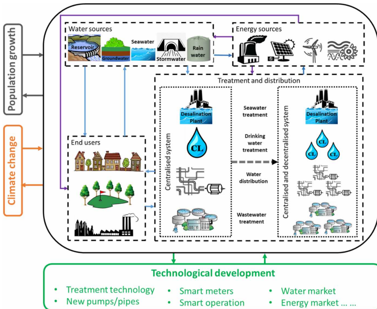
Figure 7 | Changed water–energy nexus in UWSSs due to long-term drivers. Note: Purple arrows show the flow of energy and blue arrows show the flow of water. Please refer to the online version of this paper to see this figure in colour: http://dx.doi.org/10.2166/wcc.2020.276 .
