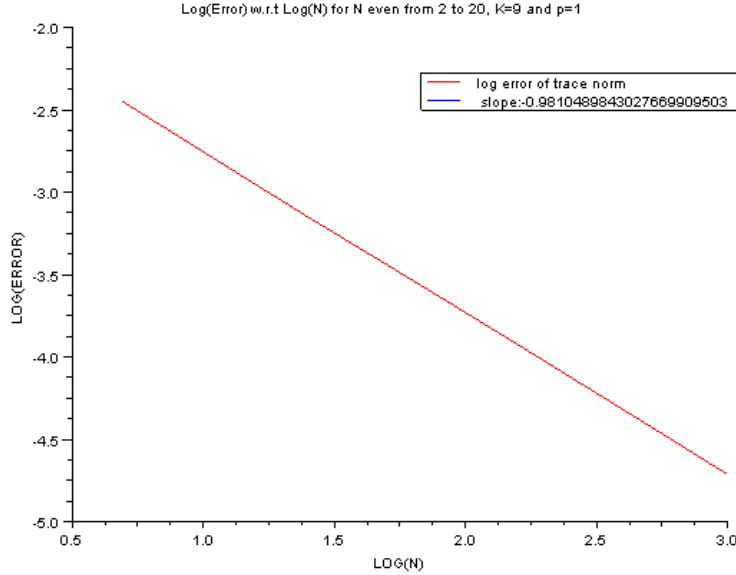
Figure 2: Log-Log plot for twin states
