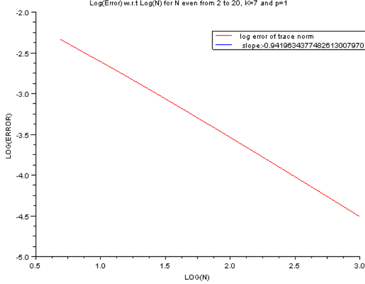
Figure 1: Log-Log plot for factorized states
