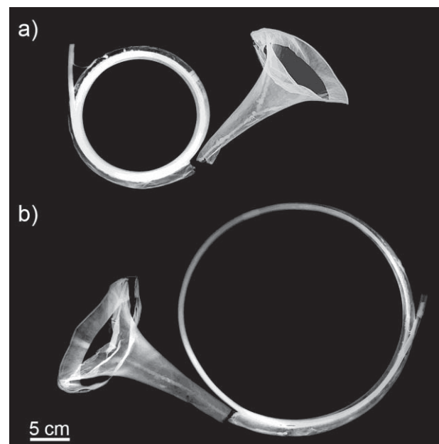
Fig. 2. X-Ray radiography respectively of the inv.878 by Johann Wilhelm Haas (a) and on the inv.877 by Wolf Wilhelm Haas (b).
