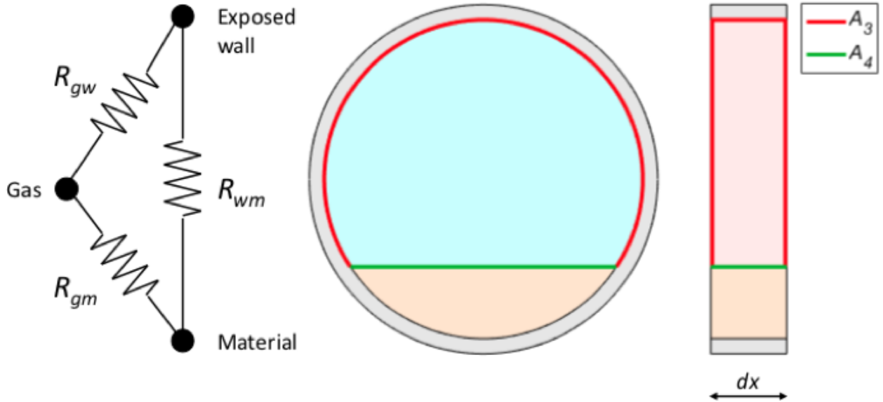
Fig. 3. Resistance network for radiative heat transfers.
