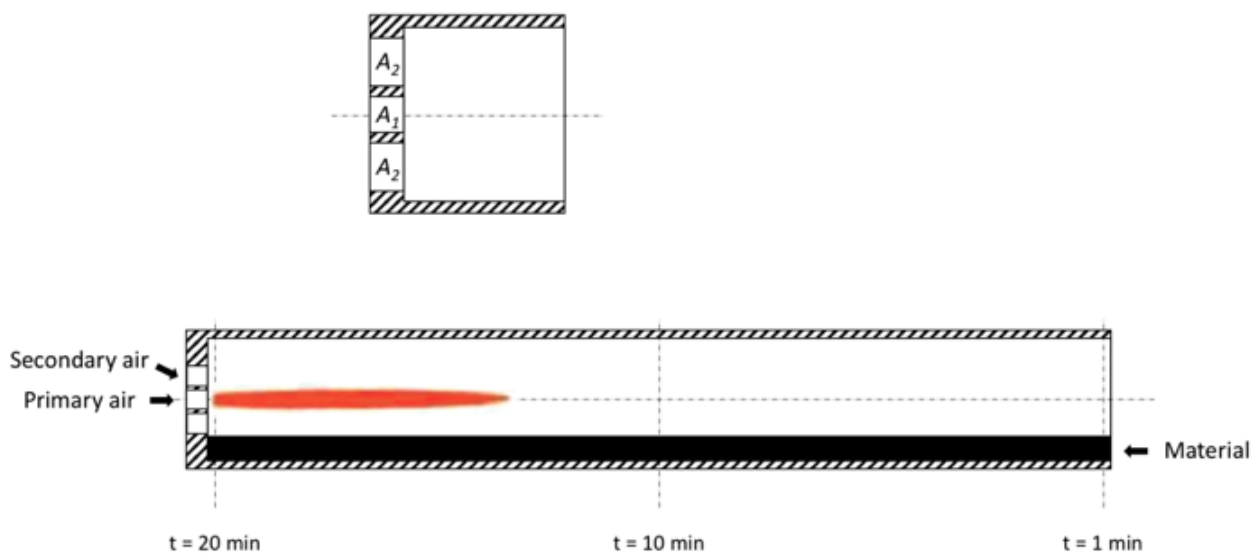
Fig. 1. Kiln geometry, detail of air-intake and positions of DEM domain at different times.
