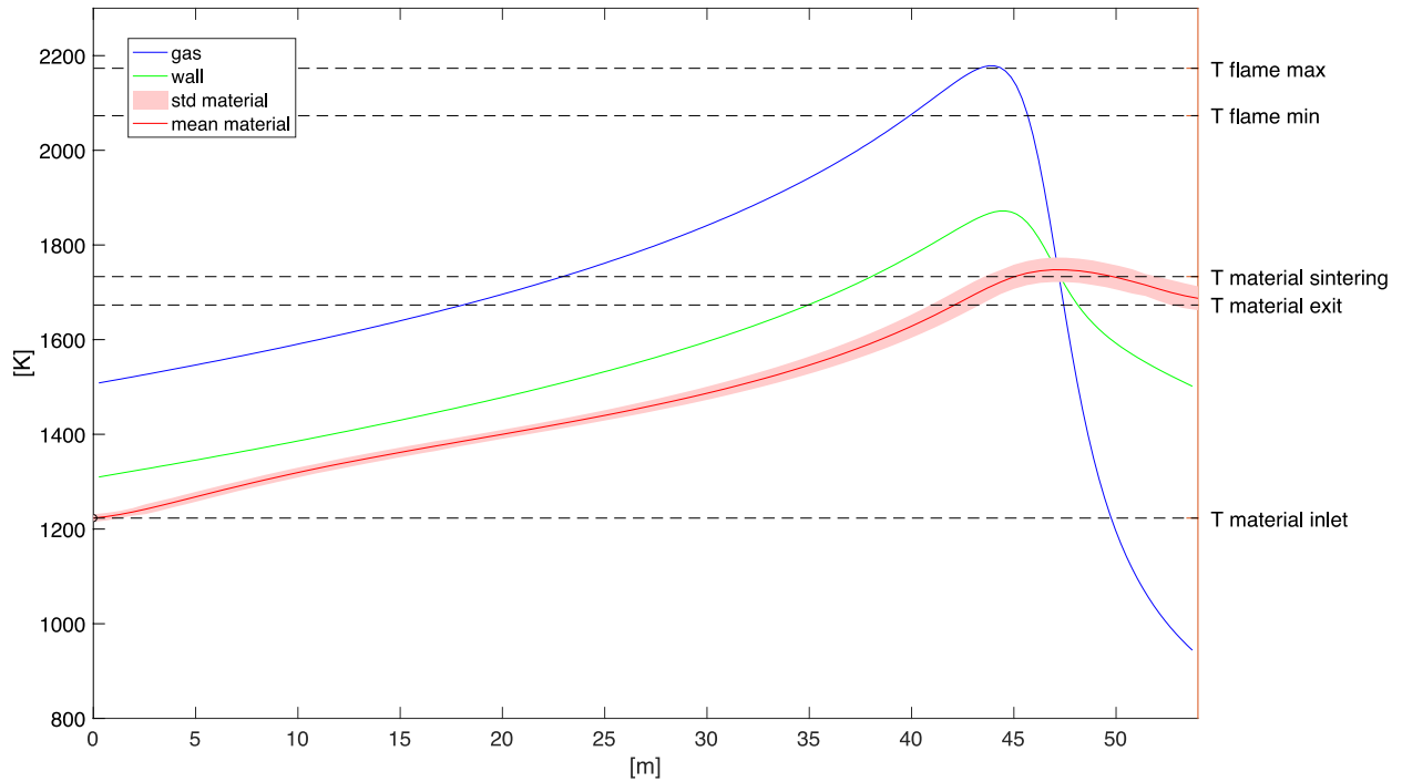
Fig. 7. Temperature profiles.
