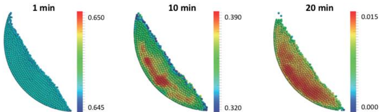
Fig. 8. CaO mass fractions at different times.
